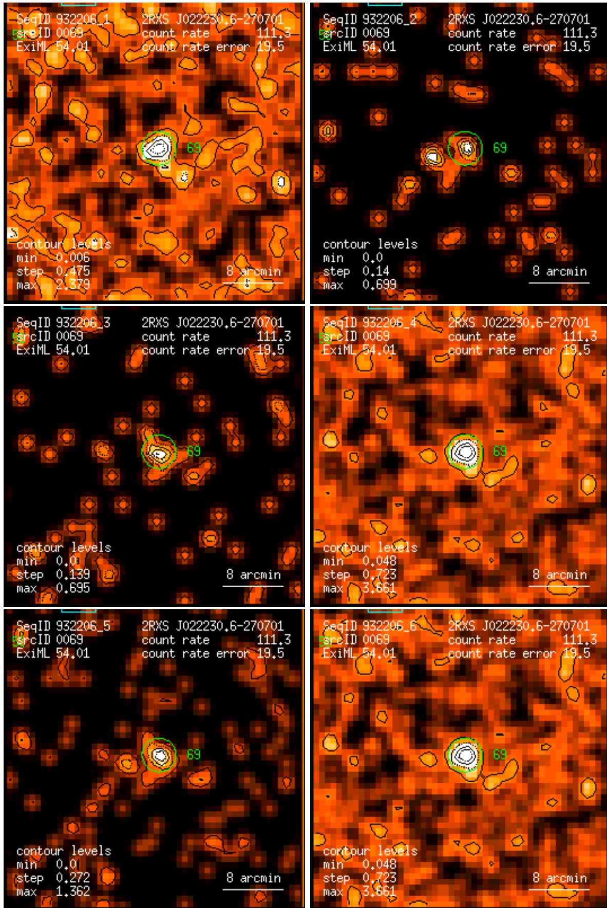
Figure 69: RASS 932206: detection 0069: band rate images, Gaussian filter: (1) PSPC channels 11 – 41, (2) 52 – 90, (3) 91 – 201, (4) 11 – 235, (5) 52 – 201, (6) 11 – 201. Broad band rates in counts/ks. Band rate contour levels in counts/ks/arcmin 2 .
