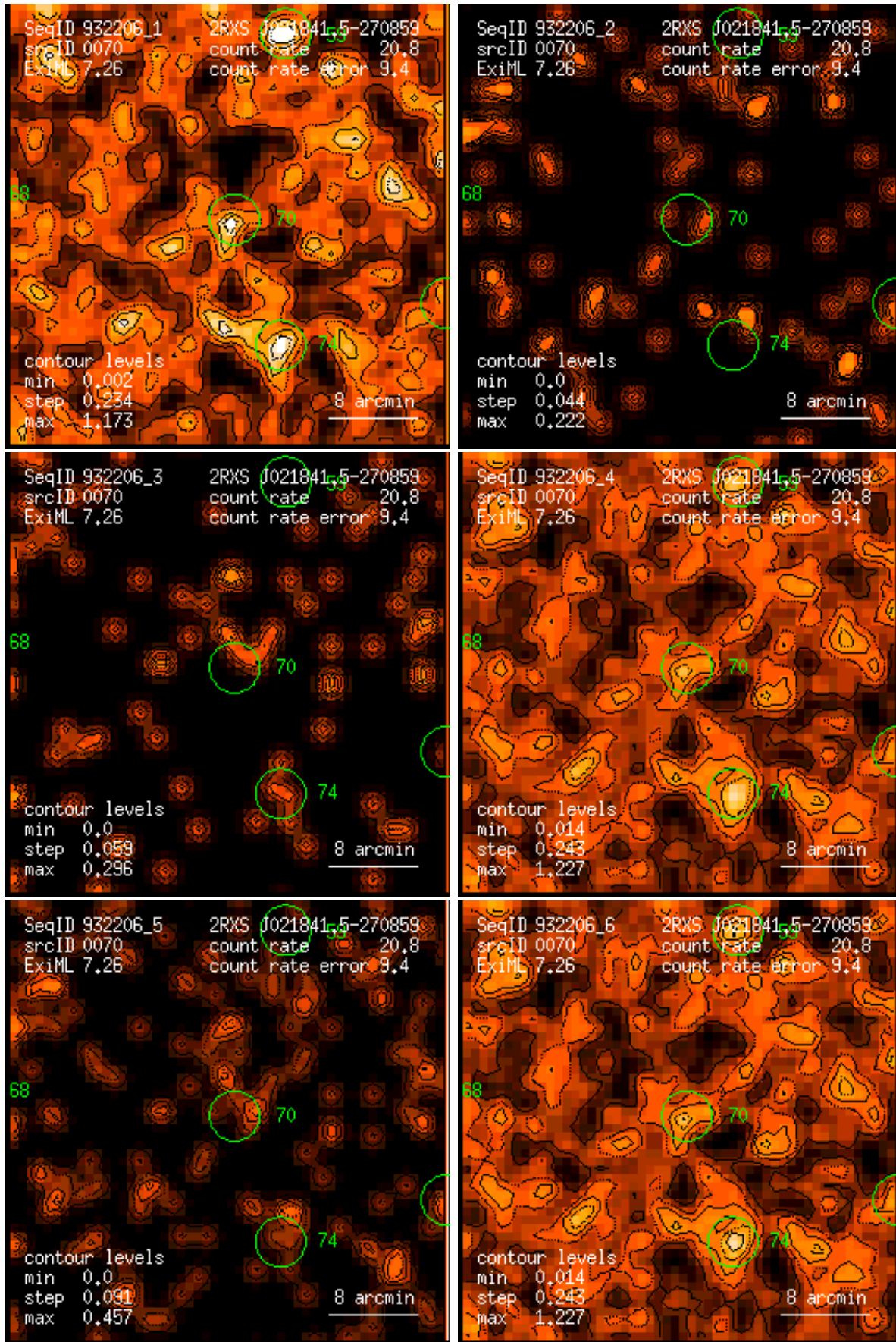
Figure 70: RASS 932206: detection 0070: band rate images, Gaussian filter: (1) PSPC channels 11 – 41, (2) 52 – 90, (3) 91 – 201, (4) 11 – 235, (5) 52 – 201, (6) 11 – 201. Broad band rates in counts/ks. Band rate contour levels in counts/ks/arcmin 2 .
