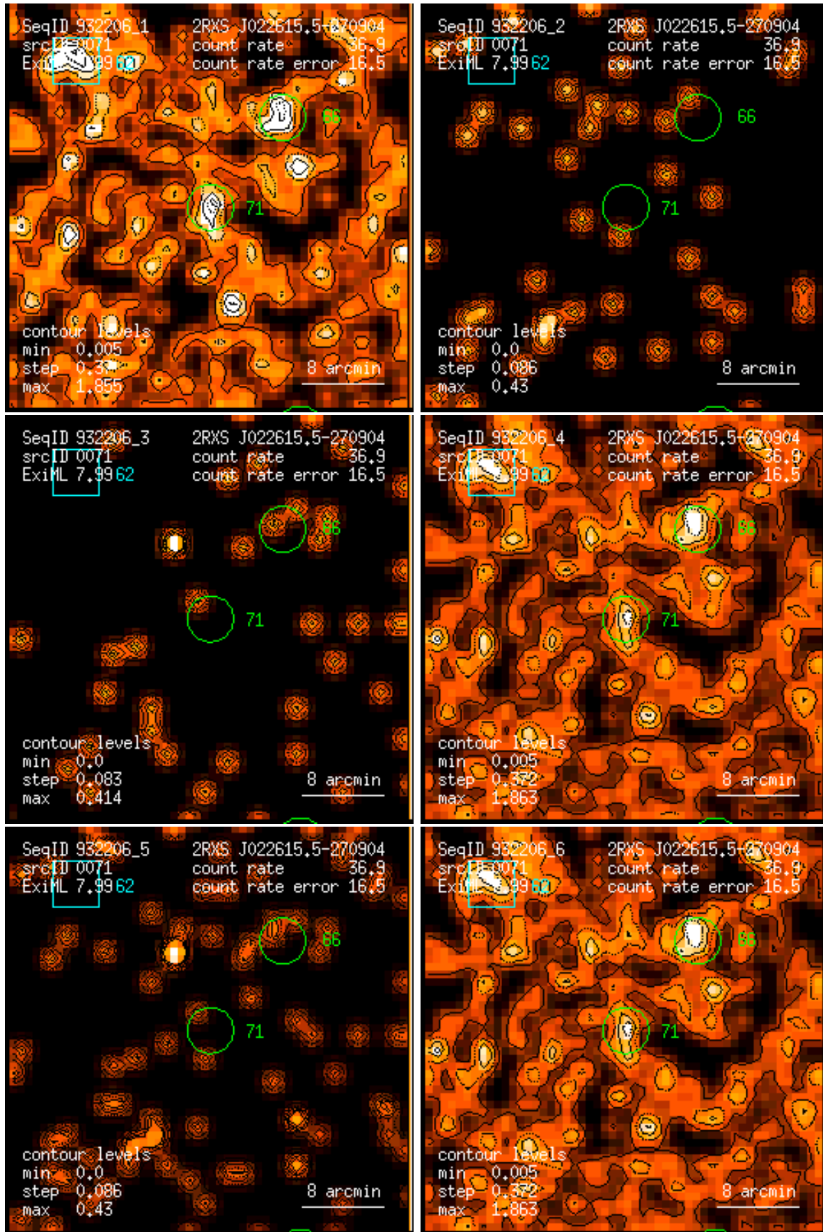
Figure 71: RASS 932206: detection 0071: band rate images, Gaussian filter: (1) PSPC channels 11 – 41, (2) 52 – 90, (3) 91 – 201, (4) 11 – 235, (5) 52 – 201, (6) 11 – 201. Broad band rates in counts/ks. Band rate contour levels in counts/ks/arcmin 2 .
