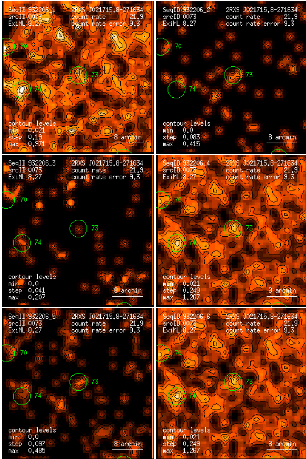
Figure 73: RASS 932206: detection 0073: band rate images, Gaussian filter: (1) PSPPC channels 11 – 41, (2) 52 – 90, (3) 91 – 201, (4) 11 – 235, (5) 52 – 201, (6) 11 – 201. Broad band rates in counts/ks. Band rate contour levels in counts/ks/arcmin 2 .
