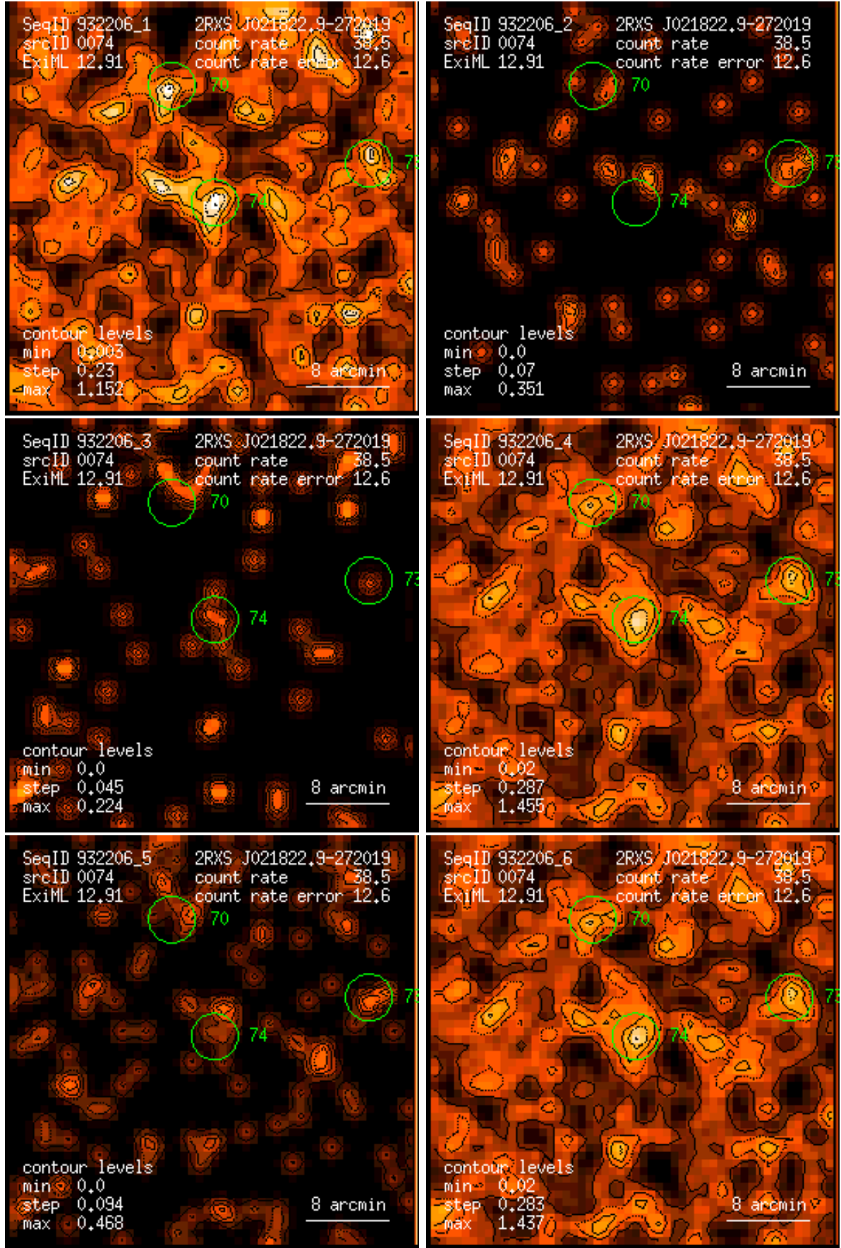
Figure 74: RASS 932206: detection 0074: band rate images, Gaussian filter: (1) PSPC channels 11 – 41, (2) 52 – 90, (3) 91 – 201, (4) 11 – 235, (5) 52 – 201, (6) 11 – 201. Broad band rates in counts/ks. Band rate contour levels in counts/ks/arcmin 2 .
