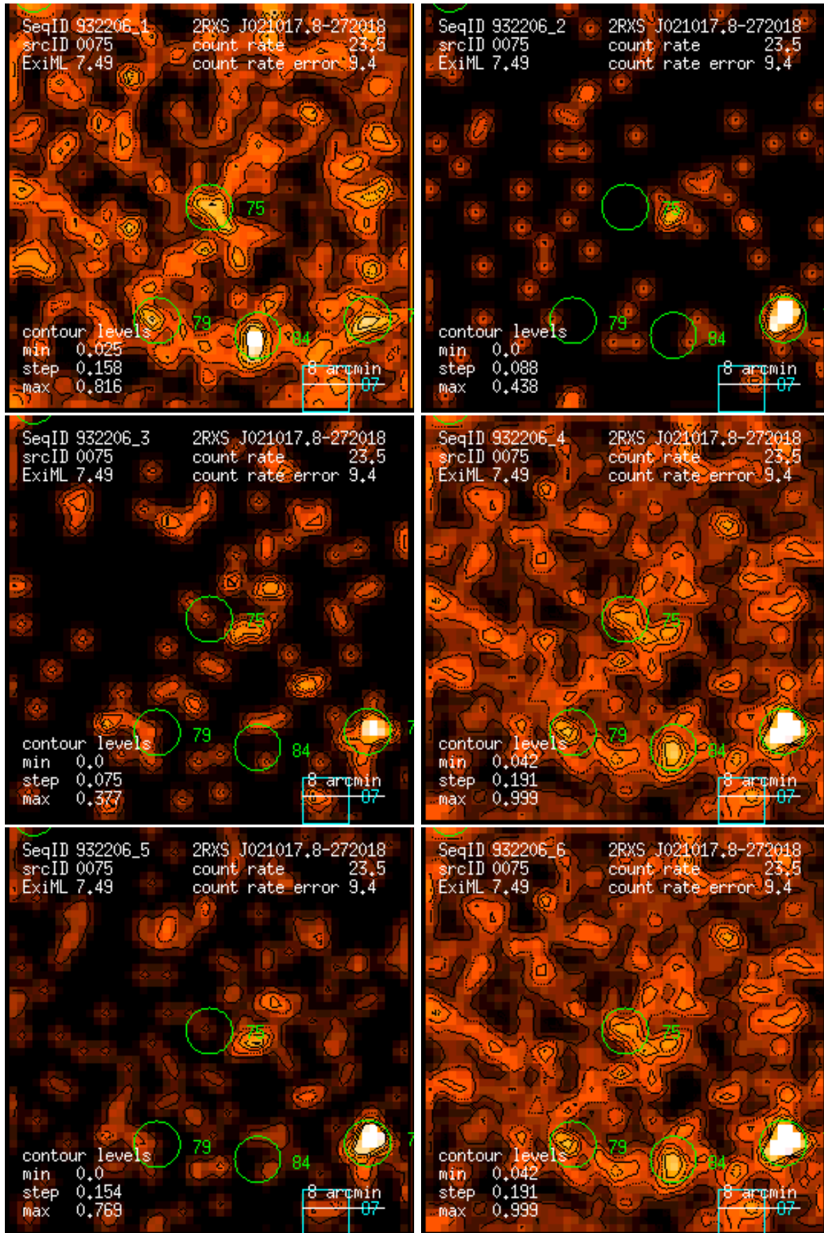
Figure 75: RASS 932206: detection 0075: band rate images, Gaussian filter: (1) PSPC channels 11 – 41, (2) 52 – 90, (3) 91 – 201, (4) 11 – 235, (5) 52 – 201, (6) 11 – 201. Broad band rates in counts/ks. Band rate contour levels in counts/ks/arcmin 2 .
