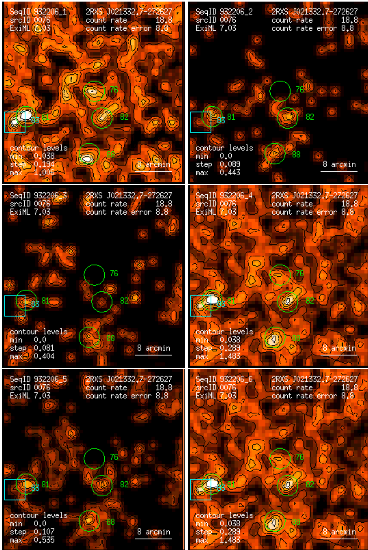
Figure 76: RASS 932206: detection 0076: band rate images, Gaussian filter: (1) PSPC channels 11 – 41, (2) 52 – 90, (3) 91 – 201, (4) 11 – 235, (5) 52 – 201, (6) 11 – 201. Broad band rates in counts/ks. Band rate contour levels in counts/ks/arcmin 2 .
