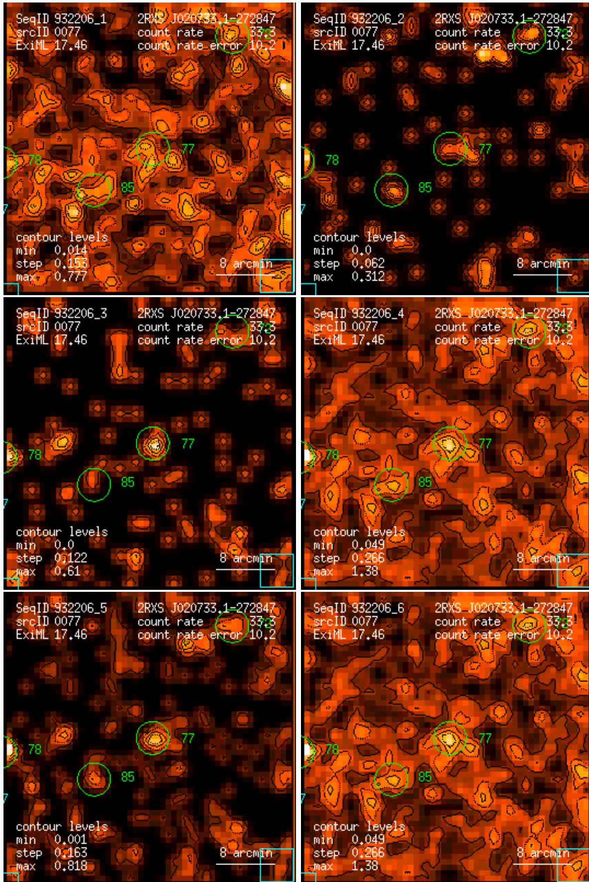
Figure 77: RASS 932206: detection 0077: band rate images, Gaussian filter: (1) PSPC channels 11 – 41, (2) 52 – 90, (3) 91 – 201, (4) 11 – 235, (5) 52 – 201, (6) 11 – 201. Broad band rates in counts/ks. Band rate contour levels in counts/ks/arcmin 2 .
