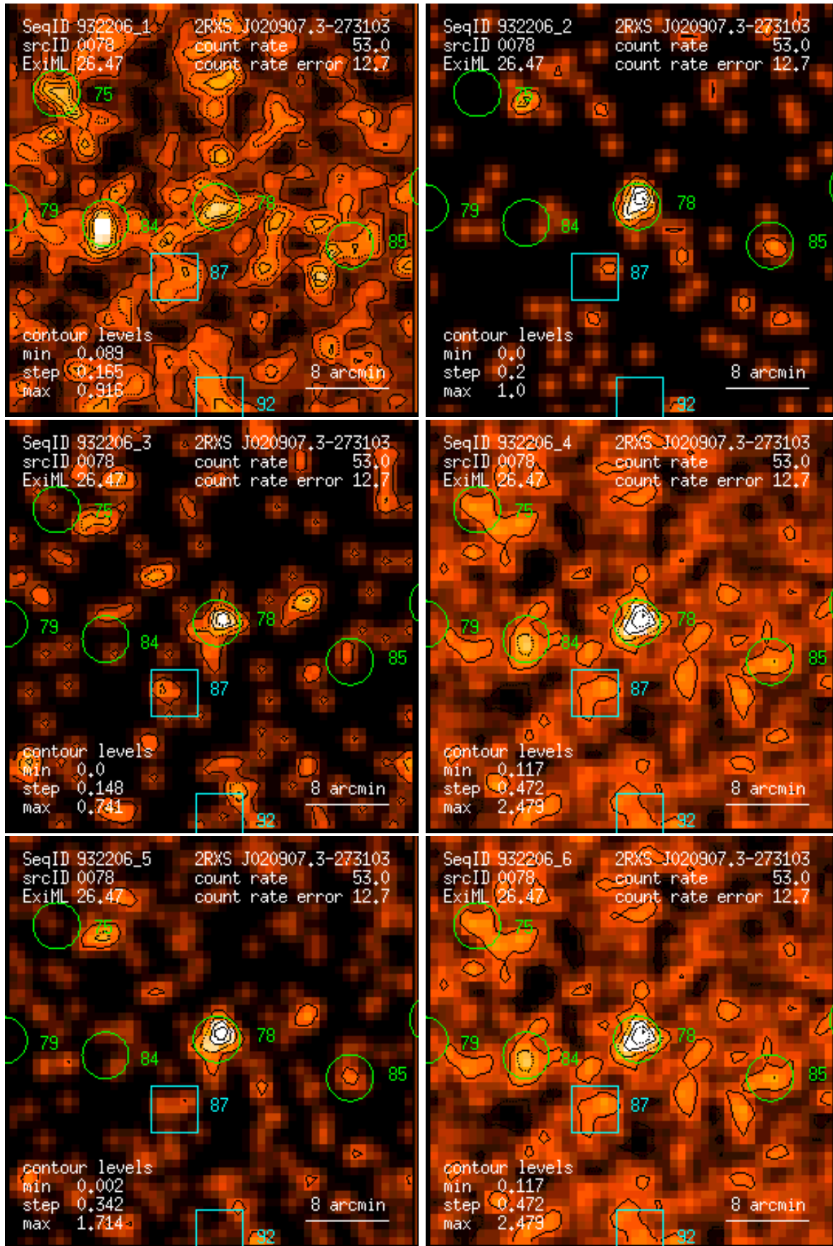
Figure 78: RASS 932206: detection 0078: band rate images, Gaussian filter: (1) PSPC channels 11 – 41, (2) 52 – 90, (3) 91 – 201, (4) 11 – 235, (5) 52 – 201, (6) 11 – 201. Broad band rates in counts/ks. Band rate contour levels in counts/ks/arcmin 2 .
