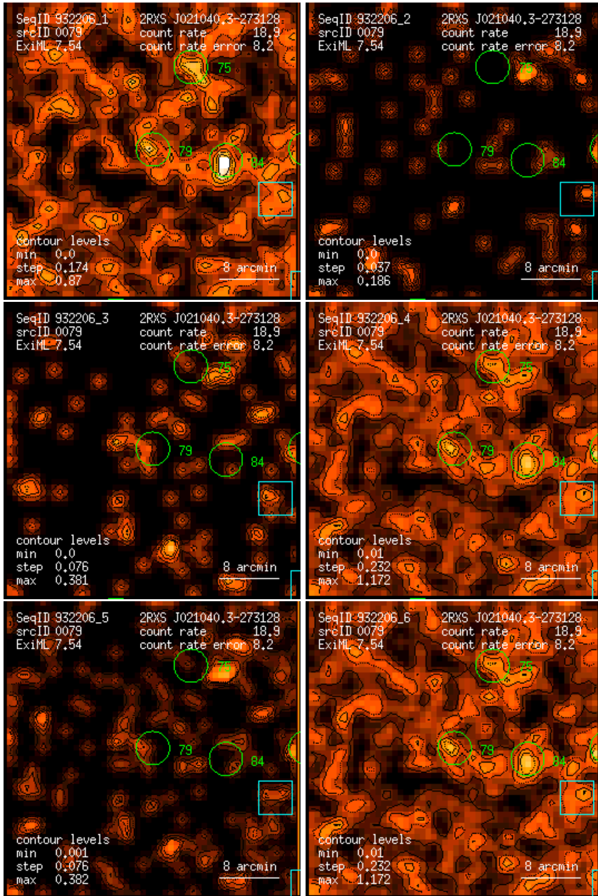
Figure 79: RASS 932206: detection 0079: band rate images, Gaussian filter: (1) PSPC channels 11 – 41, (2) 52 – 90, (3) 91 – 201, (4) 11 – 235, (5) 52 – 201, (6) 11 – 201. Broad band rates in counts/ks. Band rate contour levels in counts/ks/arcmin 2 .
