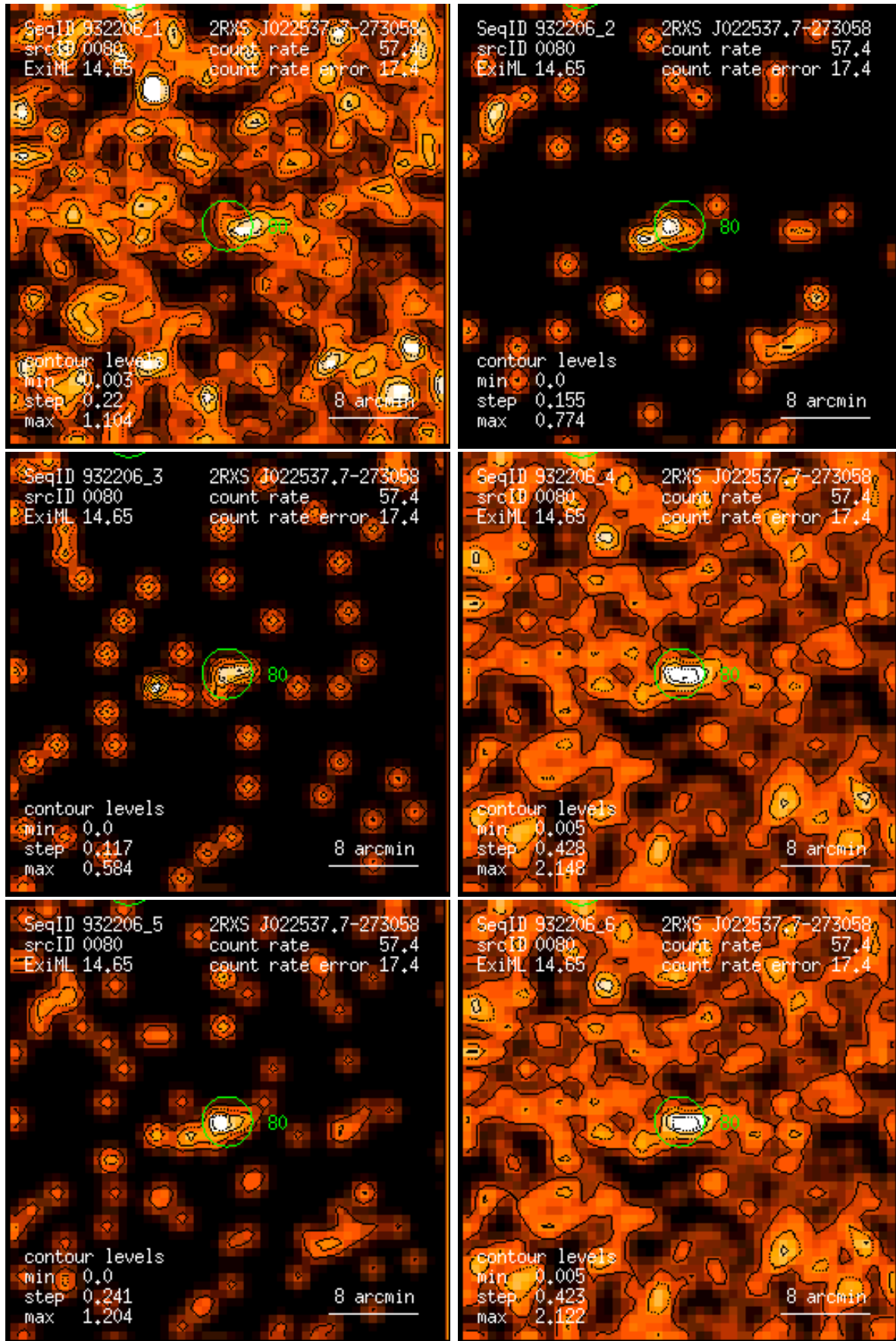
Figure 80: RASS 932206: detection 0080: band rate images, Gaussian filter: (1) PSPC channels 11 – 41, (2) 52 – 90, (3) 91 – 201, (4) 11 – 235, (5) 52 – 201, (6) 11 – 201. Broad band rates in counts/ks. Band rate contour levels in counts/ks/arcmin 2 .
