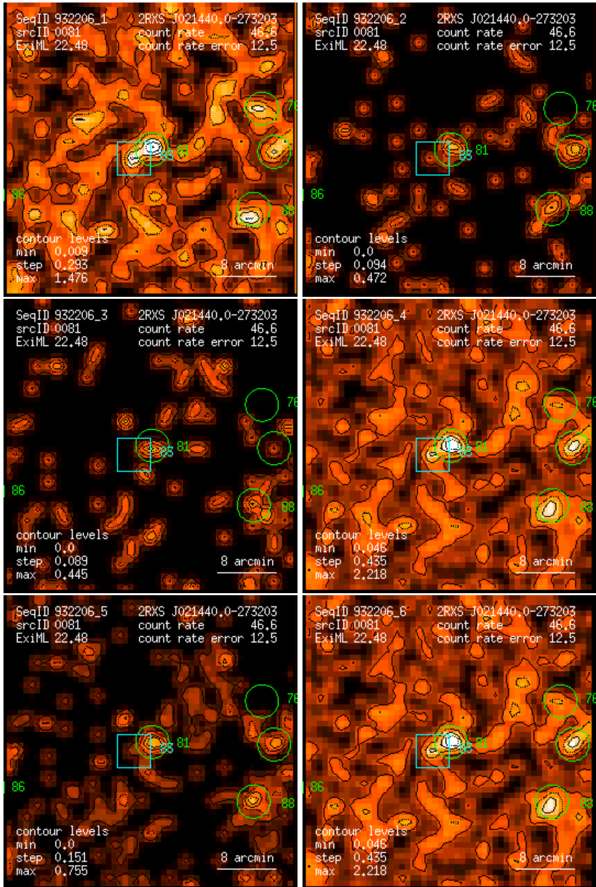
Figure 81: RASS 932206: detection 0081: band rate images, Gaussian filter: (1) PSPC channels 11 – 41, (2) 52 – 90, (3) 91 – 201, (4) 11 – 235, (5) 52 – 201, (6) 11 – 201. Broad band rates in counts/ks. Band rate contour levels in counts/ks/arcmin 2 .
