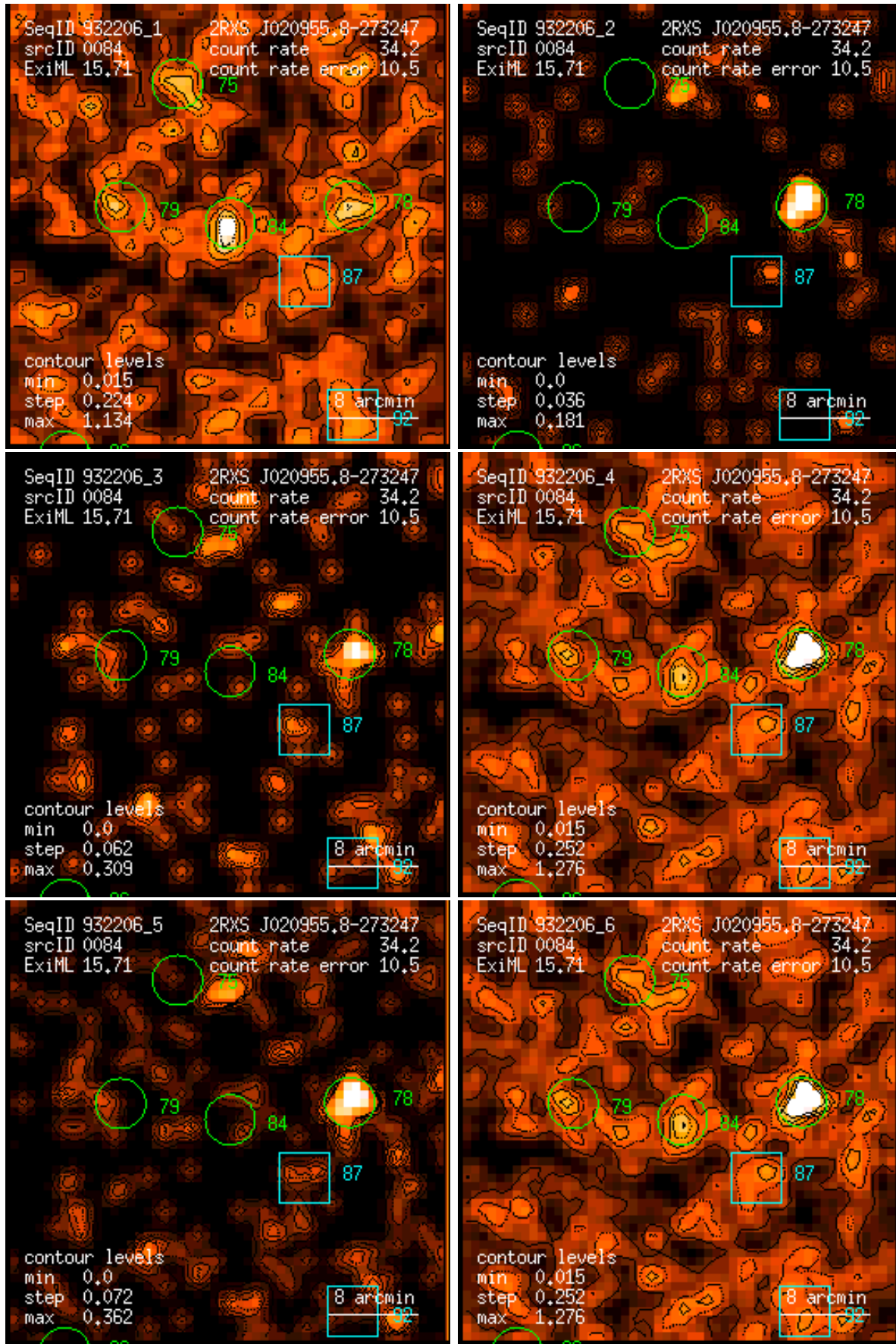
Figure 84: RASS 932206: detection 0084: band rate images, Gaussian filter: (1) PSPC channels 11 – 41, (2) 52 – 90, (3) 91 – 201, (4) 11 – 235, (5) 52 – 201, (6) 11 – 201. Broad band rates in counts/ks. Band rate contour levels in counts/ks/arcmin 2 .
