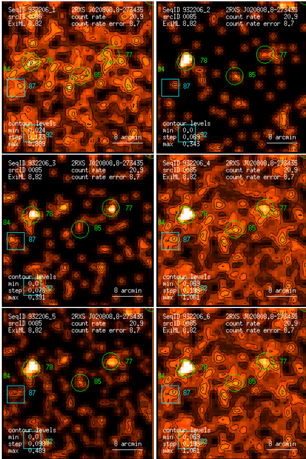
Figure 85: RASS 932206: detection 0085: band rate images, Gaussian filter: (1) PSPC channels 11 – 41, (2) 52 – 90, (3) 91 – 201, (4) 11 – 235, (5) 52 – 201, (6) 11 – 201. Broad band rates in counts/ks. Band rate contour levels in counts/ks/arcmin 2 .
