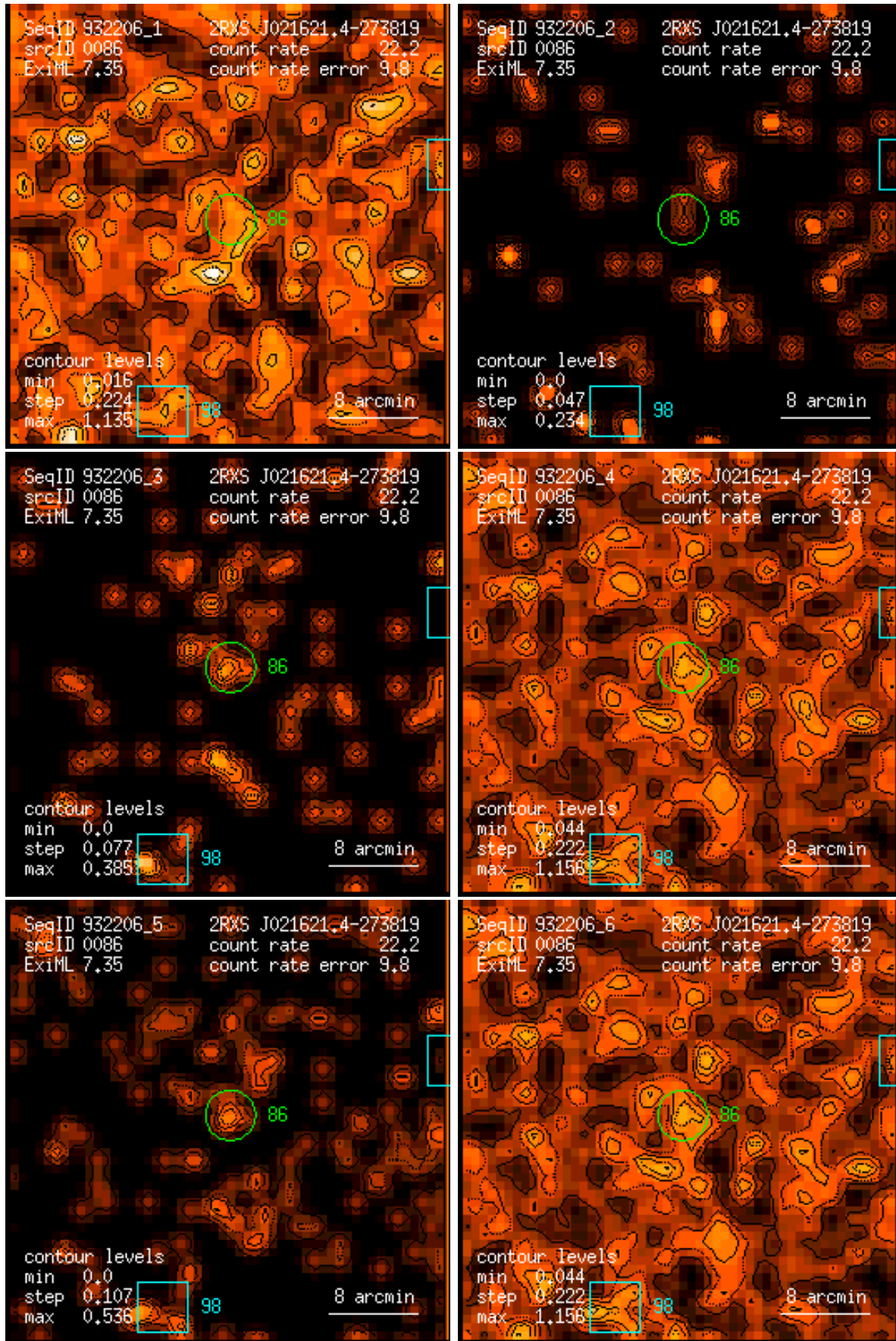
Figure 86: RASS 932206: detection 0086: band rate images, Gaussian filter: (1) PSPC channels 11 – 41, (2) 52 – 90, (3) 91 – 201, (4) 11 – 235, (5) 52 – 201, (6) 11 – 201. Broad band rates in counts/ks. Band rate contour levels in counts/ks/arcmin 2 .
