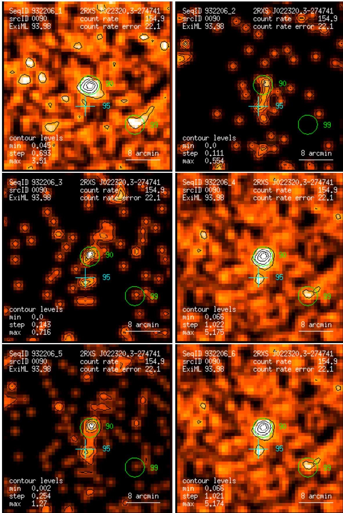
Figure 90: RASS 932206: detection 0090: band rate images, Gaussian filter: (1) PSPC channels 11 – 41, (2) 52 – 90, (3) 91 – 201, (4) 11 – 235, (5) 52 – 201, (6) 11 – 201. Broad band rates in counts/ks. Band rate contour levels in counts/ks/arcmin 2 .
