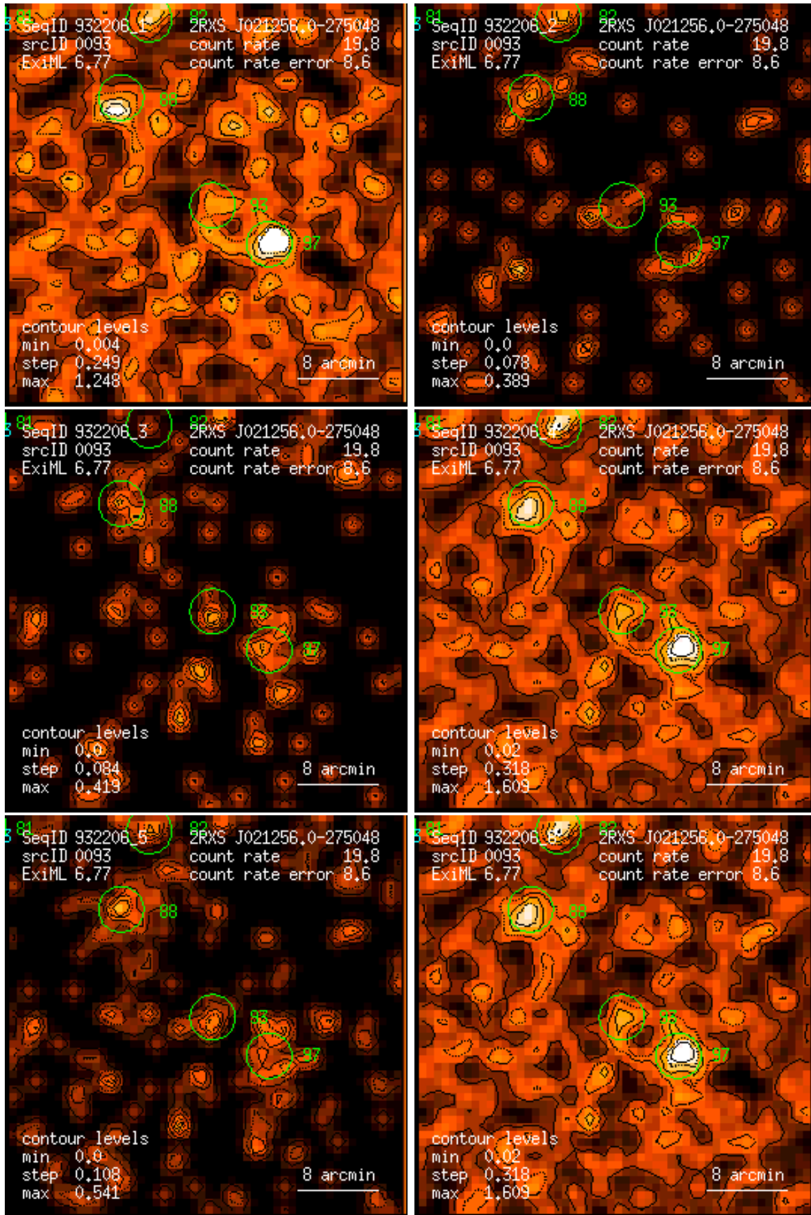
Figure 93: RASS 932206: detection 0093: band rate images, Gaussian filter: (1) PSPC channels 11 – 41, (2) 52 – 90, (3) 91 – 201, (4) 11 – 235, (5) 52 – 201, (6) 11 – 201. Broad band rates in counts/ks. Band rate contour levels in counts/ks/arcmin 2 .
