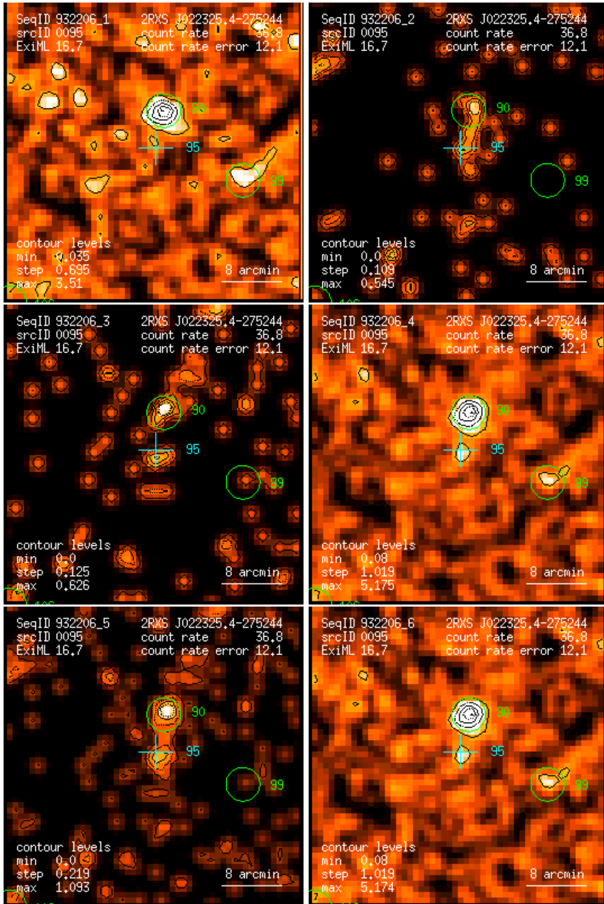
Figure 95: RASS 932206: detection 0095: band rate images, Gaussian filter: (1) PSPC channels 11 – 41, (2) 52 – 90, (3) 91 – 201, (4) 11 – 235, (5) 52 – 201, (6) 11 – 201. Broad band rates in counts/ks. Band rate contour levels in counts/ks/arcmin 2 .
