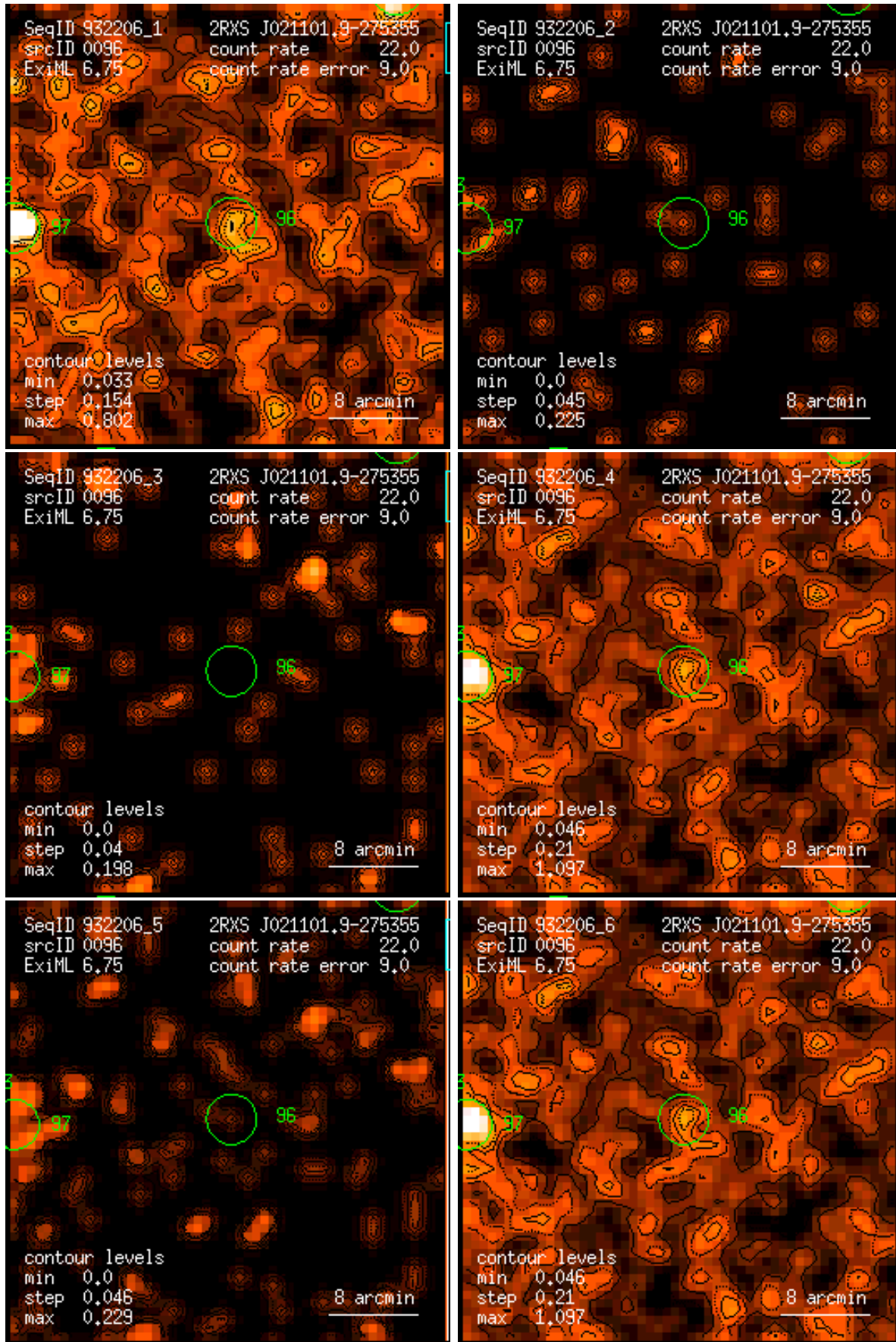
Figure 96: RASS 932206: detection 0096: band rate images, Gaussian filter: (1) PSPC channels 11 – 41, (2) 52 – 90, (3) 91 – 201, (4) 11 – 235, (5) 52 – 201, (6) 11 – 201. Broad band rates in counts/ks. Band rate contour levels in counts/ks/arcmin 2 .
