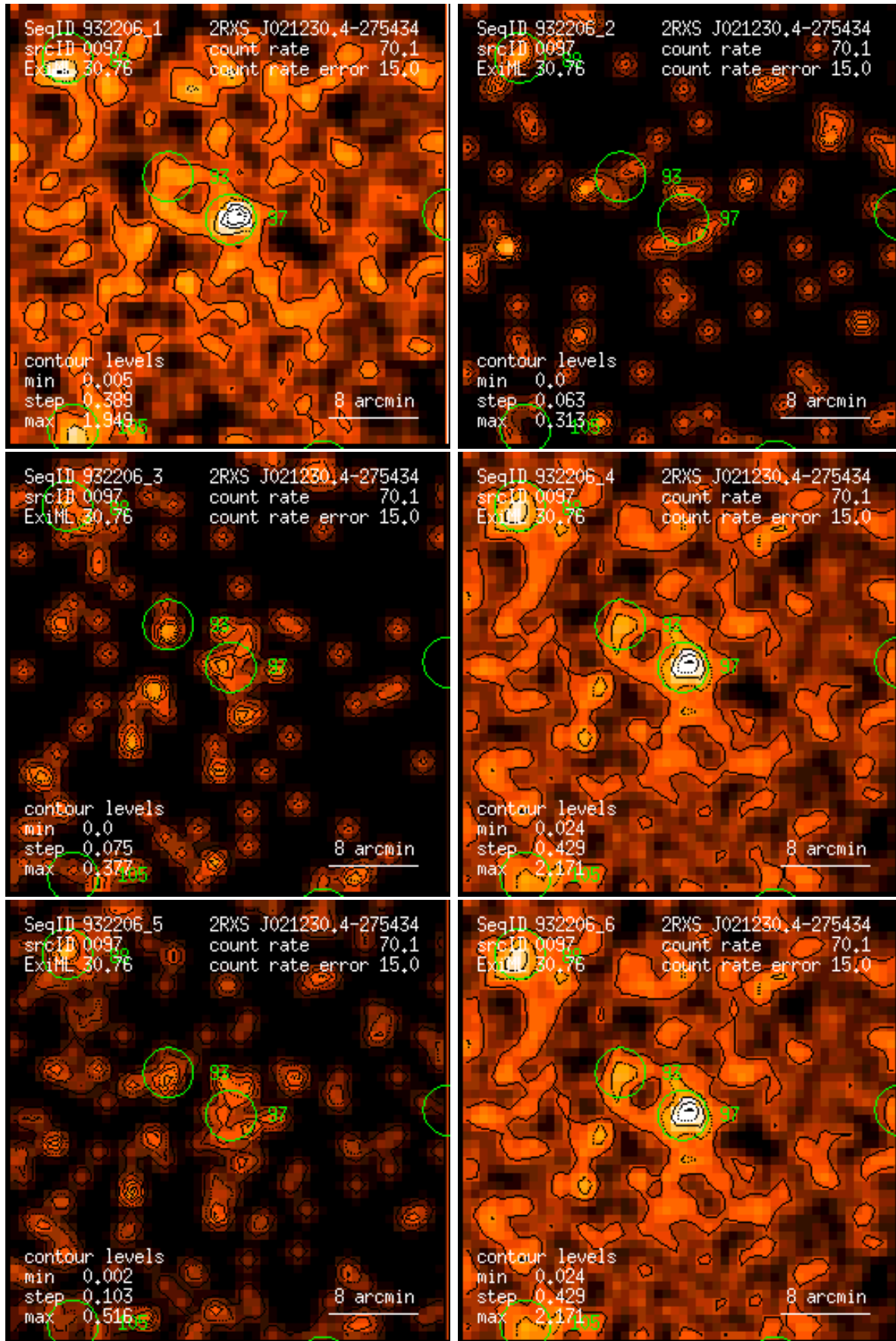
Figure 97: RASS 932206: detection 0097: band rate images, Gaussian filter: (1) PSPC channels 11 – 41, (2) 52 – 90, (3) 91 – 201, (4) 11 – 235, (5) 52 – 201, (6) 11 – 201. Broad band rates in counts/ks. Band rate contour levels in counts/ks/arcmin 2 .
