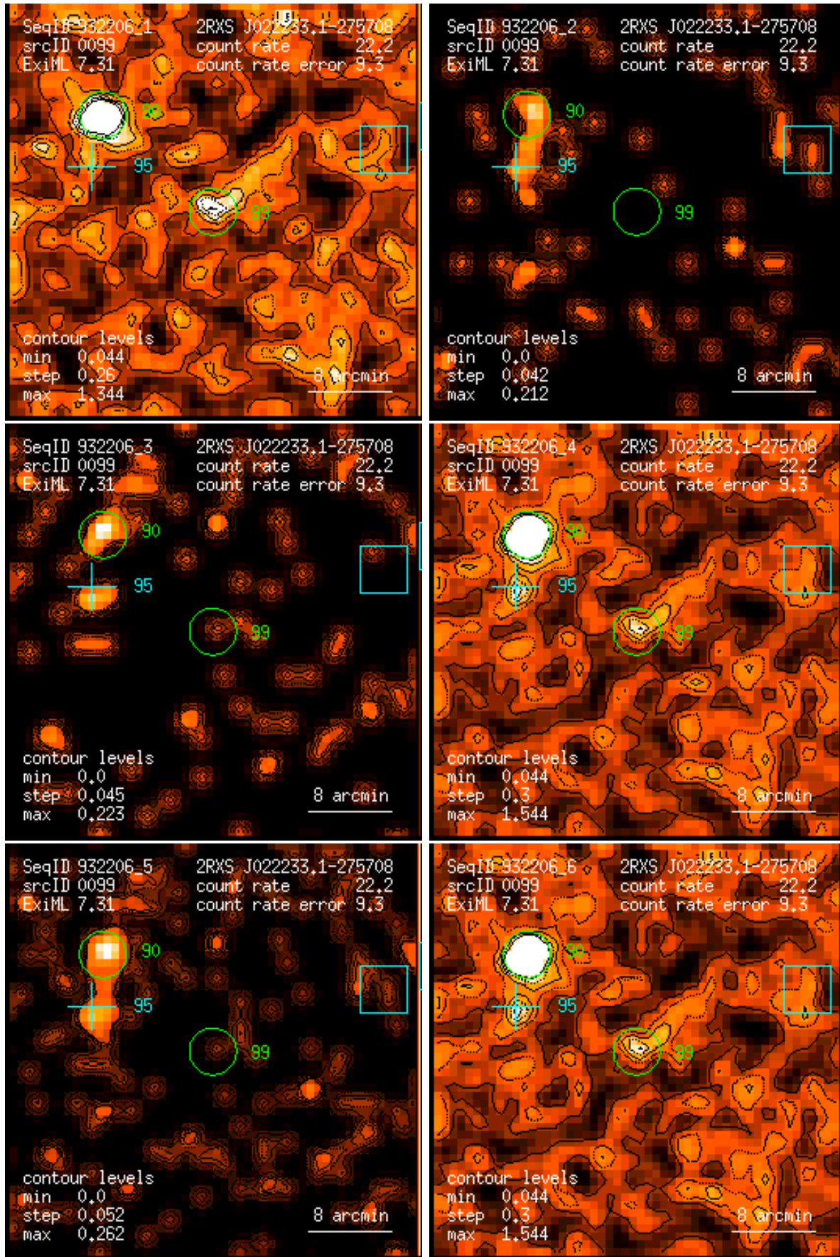
Figure 99: RASS 932206: detection 0099: band rate images, Gaussian filter: (1) PSPC channels 11 – 41, (2) 52 – 90, (3) 91 – 201, (4) 11 – 235, (5) 52 – 201, (6) 11 – 201. Broad band rates in counts/ks. Band rate contour levels in counts/ks/arcmin 2 .
