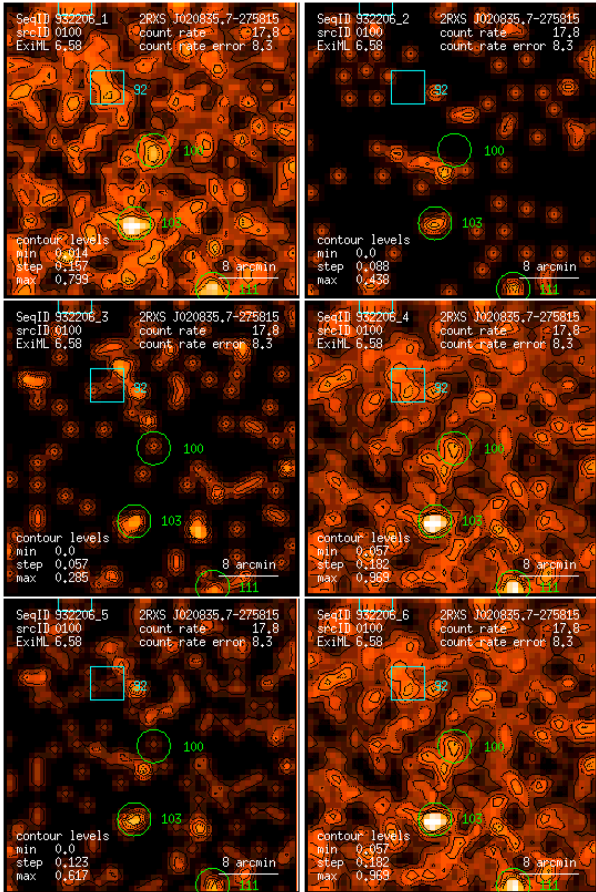
Figure 100: RASS 932206: detection 0100: band rate images, Gaussian filter: (1) PSPC channels 11 – 41, (2) 52 – 90, (3) 91 – 201, (4) 11 – 235, (5) 52 – 201, (6) 11 – 201. Broad band rates in counts/ks. Band rate contour levels in counts/ks/arcmin 2 .
