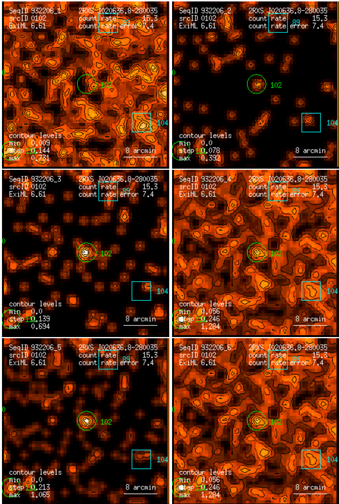
Figure 102: RASS 932206: detection 0102: band rate images, Gaussian filter: (1) PSPC channels 11 – 41, (2) 52 – 90, (3) 91 – 201, (4) 11 – 235, (5) 52 – 201, (6) 11 – 201. Broad band rates in counts/ks. Band rate contour levels in counts/ks/arcmin 2 .
