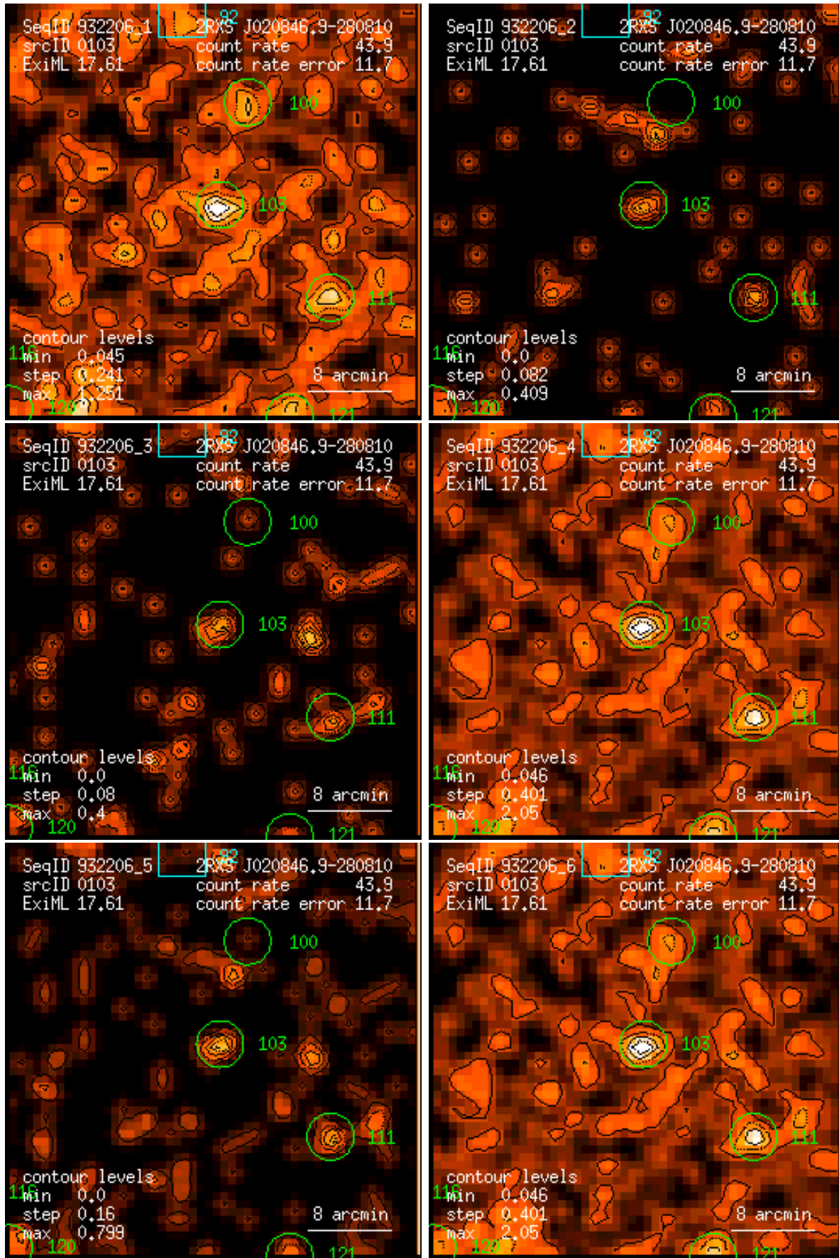
Figure 103: RASS 932206: detection 0103: band rate images, Gaussian filter: (1) PSPC channels 11 – 41, (2) 52 – 90, (3) 91 – 201, (4) 11 – 235, (5) 52 – 201, (6) 11 – 201. Broad band rates in counts/ks. Band rate contour levels in counts/ks/arcmin 2 .
