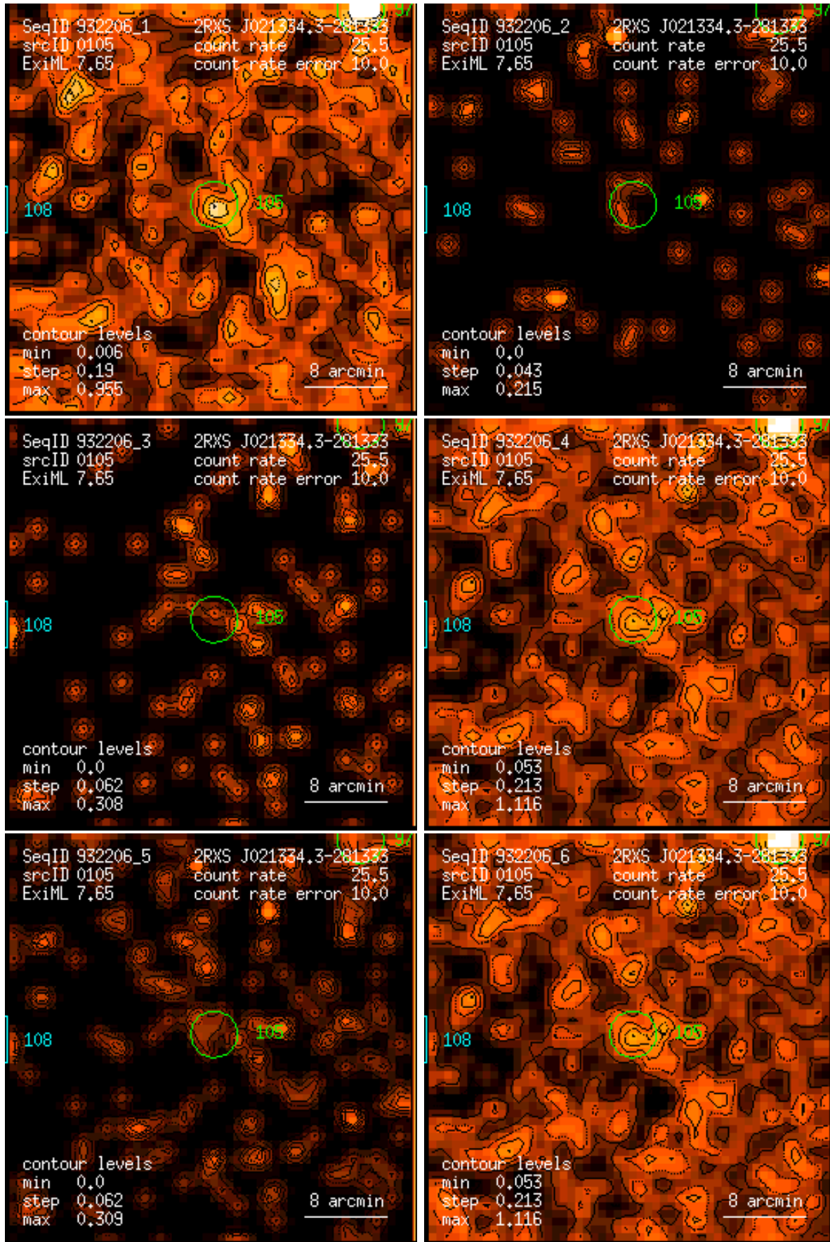
Figure 105: RASS 932206: detection 0105: band rate images, Gaussian filter: (1) PSPC channels 11 – 41, (2) 52 – 90, (3) 91 – 201, (4) 11 – 235, (5) 52 – 201, (6) 11 – 201. Broad band rates in counts/ks. Band rate contour levels in counts/ks/arcmin 2 .
