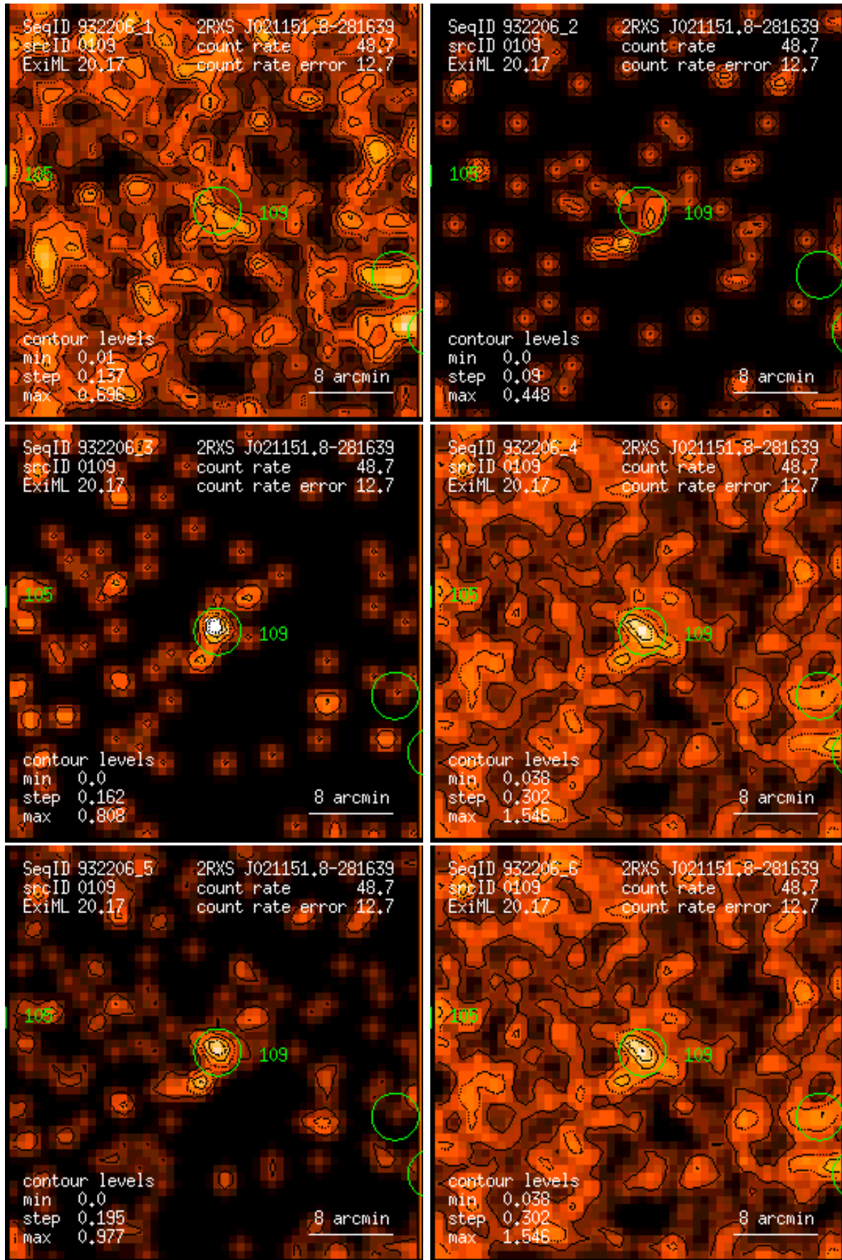
Figure 109: RASS 932206: detection 0109: band rate images, Gaussian filter: (1) PSPC channels 11 – 41, (2) 52 – 90, (3) 91 – 201, (4) 11 – 235, (5) 52 – 201, (6) 11 – 201. Broad band rates in counts/ks. Band rate contour levels in counts/ks/arcmin 2 .
