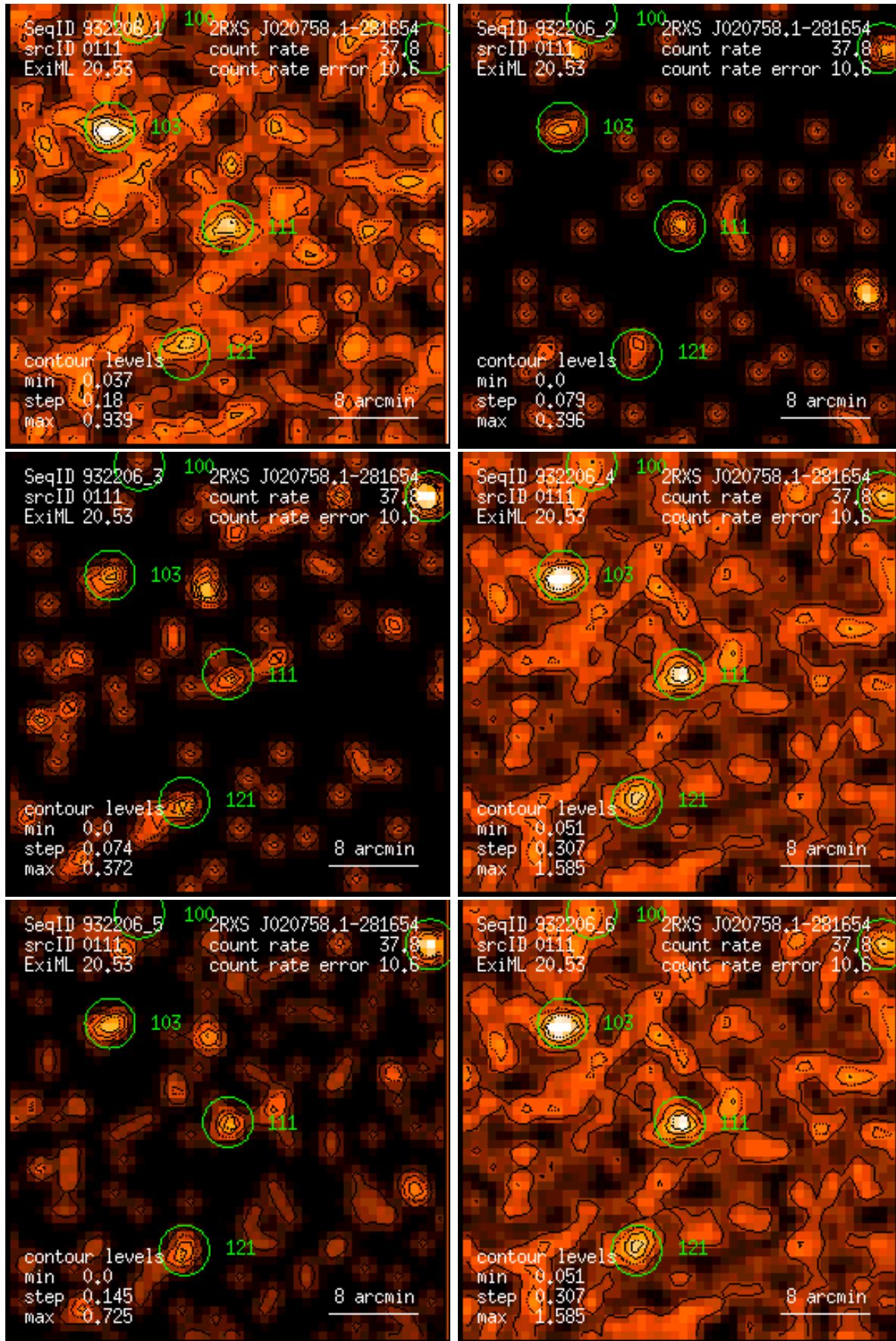
Figure 111: RASS 932206: detection 0111: band rate images, Gaussian filter: (1) PSPC channels 11 – 41, (2) 52 – 90, (3) 91 – 201, (4) 11 – 235, (5) 52 – 201, (6) 11 – 201. Broad band rates in counts/ks. Band rate contour levels in counts/ks/arcmin 2 .
