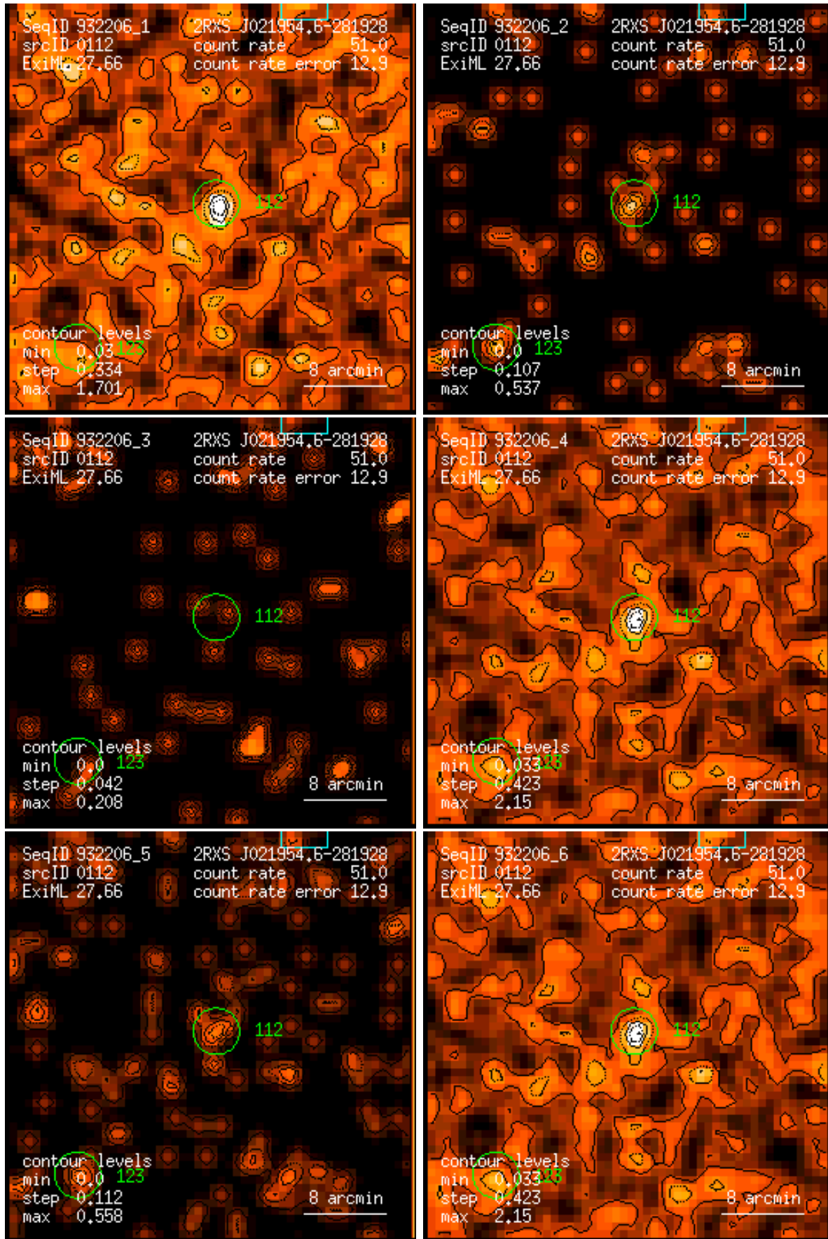
Figure 112: RASS 932206: detection 0112: band rate images, Gaussian filter: (1) PSPC channels 11 – 41, (2) 52 – 90, (3) 91 – 201, (4) 11 – 235, (5) 52 – 201, (6) 11 – 201. Broad band rates in counts/ks. Band rate contour levels in counts/ks/arcmin 2 .
