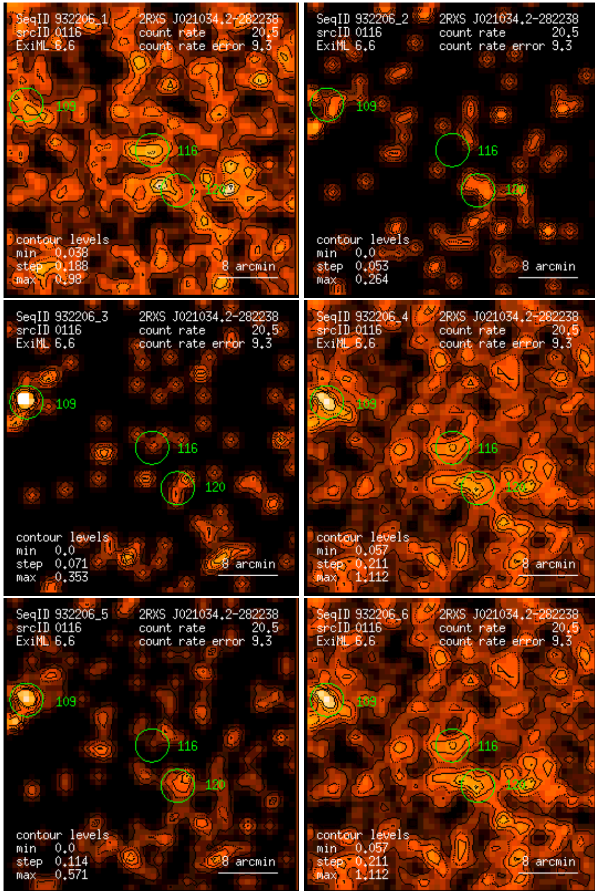
Figure 116: RASS 932206: detection 0116: band rate images, Gaussian filter: (1) PSPC channels 11 – 41, (2) 52 – 90, (3) 91 – 201, (4) 11 – 235, (5) 52 – 201, (6) 11 – 201. Broad band rates in counts/ks. Band rate contour levels in counts/ks/arcmin 2 .
