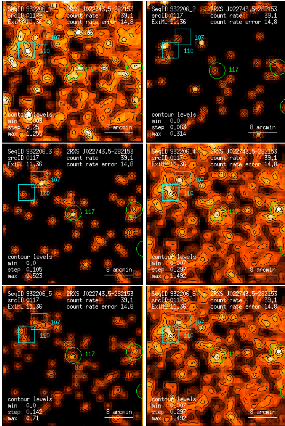
Figure 117: RASS 932206: detection 0117: band rate images, Gaussian filter: (1) PSPC channels 11 – 41, (2) 52 – 90, (3) 91 – 201, (4) 11 – 235, (5) 52 – 201, (6) 11 – 201. Broad band rates in counts/ks. Band rate contour levels in counts/ks/arcmin 2 .
