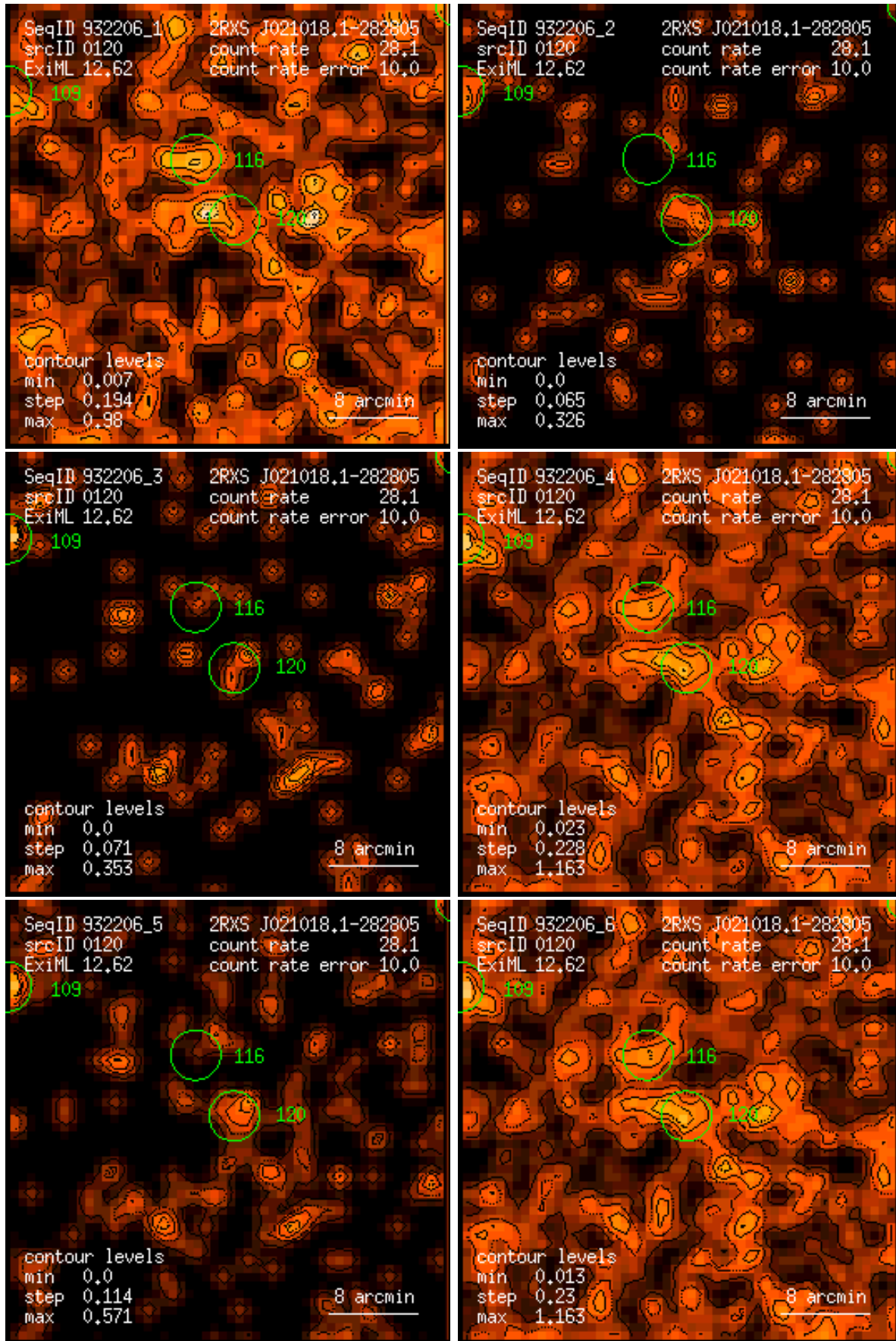
Figure 120: RASS 932206: detection 0120: band rate images, Gaussian filter: (1) PSPC channels 11 – 41, (2) 52 – 90, (3) 91 – 201, (4) 11 – 235, (5) 52 – 201, (6) 11 – 201. Broad band rates in counts/ks. Band rate contour levels in counts/ks/arcmin 2 .
