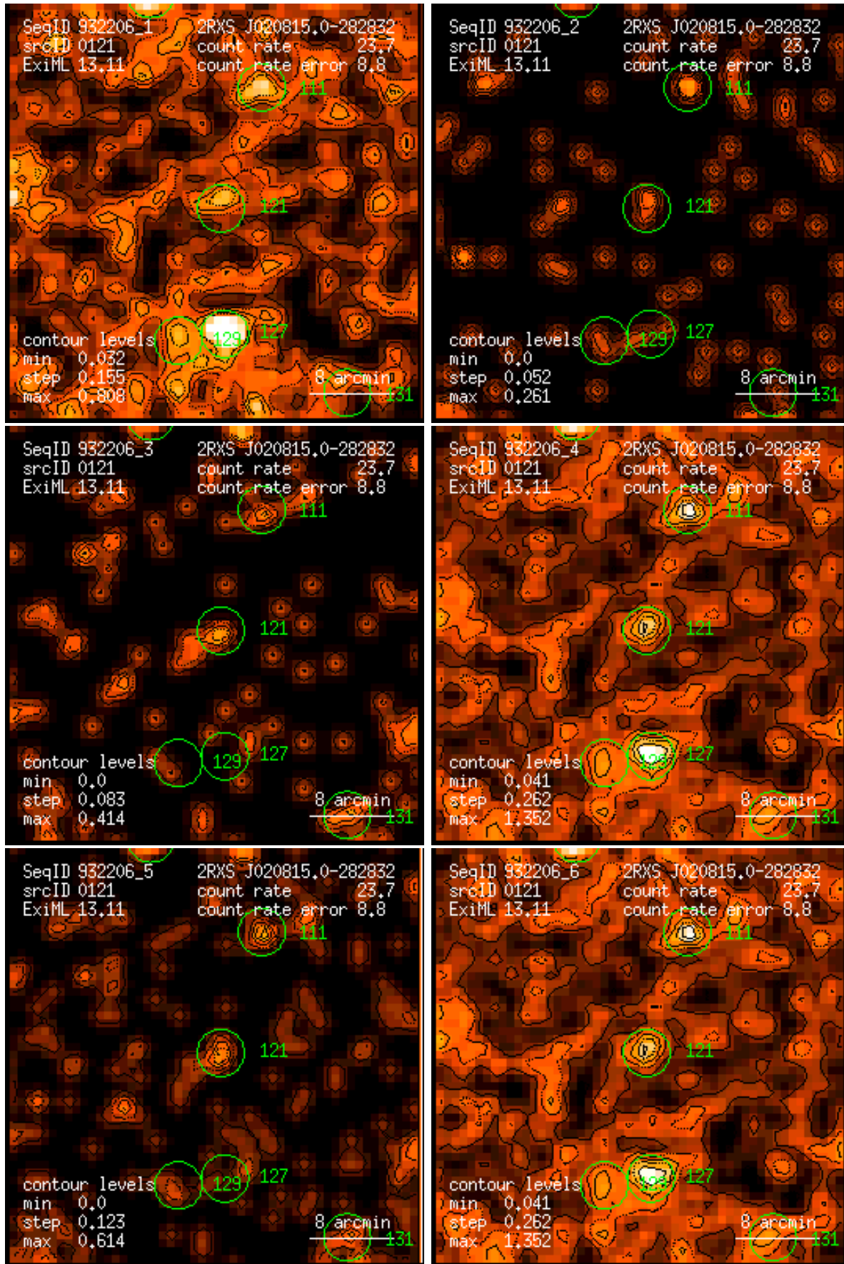
Figure 121: RASS 932206: detection 0121: band rate images, Gaussian filter: (1) PSPC channels 11 – 41, (2) 52 – 90, (3) 91 – 201, (4) 11 – 235, (5) 52 – 201, (6) 11 – 201. Broad band rates in counts/ks. Band rate contour levels in counts/ks/arcmin 2 .
