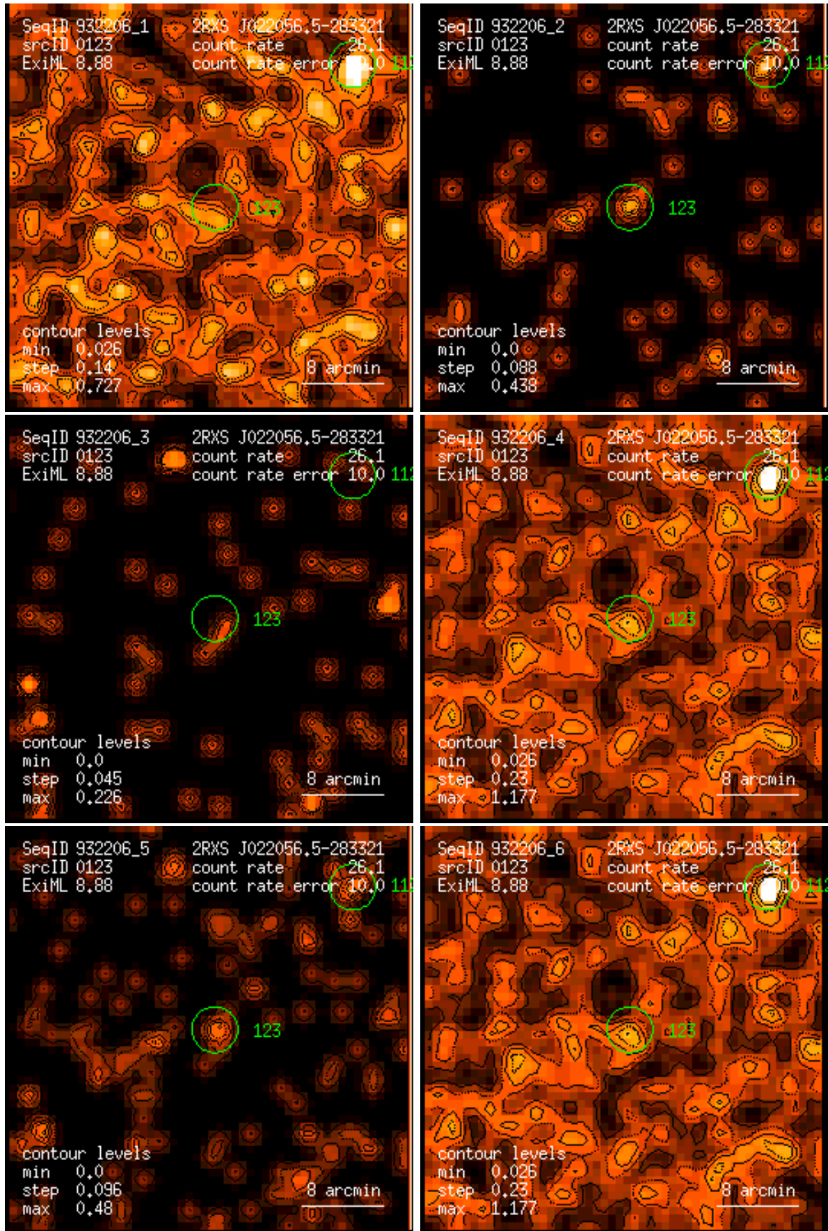
Figure 123: RASS 932206: detection 0123: band rate images, Gaussian filter: (1) PSPC channels 11 – 41, (2) 52 – 90, (3) 91 – 201, (4) 11 – 235, (5) 52 – 201, (6) 11 – 201. Broad band rates in counts/ks. Band rate contour levels in counts/ks/arcmin 2 .
