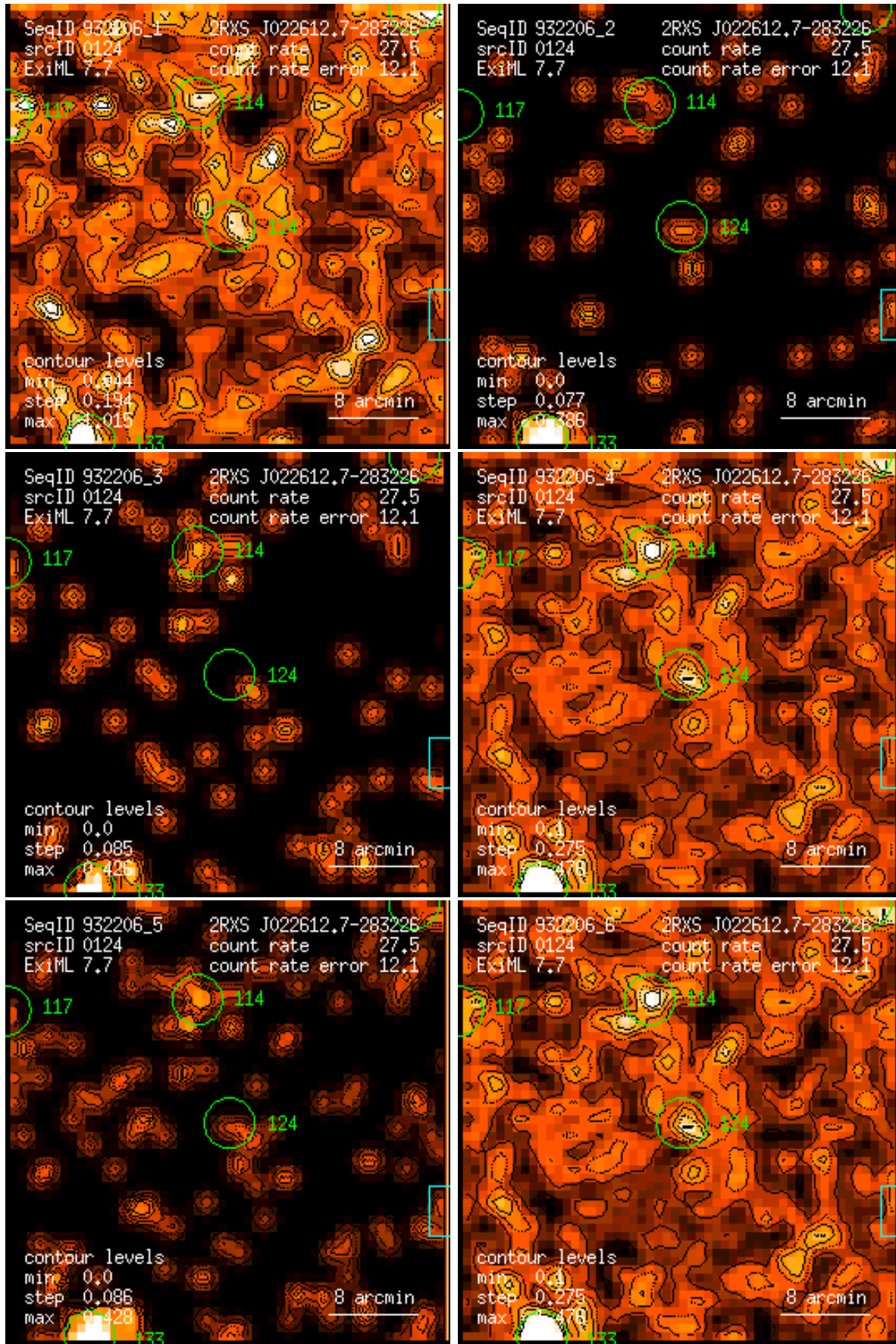
Figure 124: RASS 932206: detection 0124: band rate images, Gaussian filter: (1) PSPC channels 11 – 41, (2) 52 – 90, (3) 91 – 201, (4) 11 – 235, (5) 52 – 201, (6) 11 – 201. Broad band rates in counts/ks. Band rate contour levels in counts/ks/arcmin 2 .
