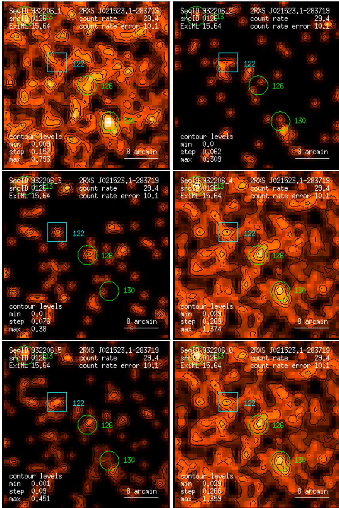
Figure 126: RASS 932206: detection 0126: band rate images, Gaussian filter: (1) PSPC channels 11 – 41, (2) 52 – 90, (3) 91 – 201, (4) 11 – 235, (5) 52 – 201, (6) 11 – 201. Broad band rates in counts/ks. Band rate contour levels in counts/ks/arcmin 2 .
