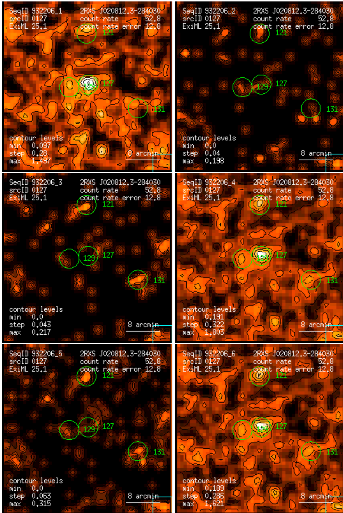
Figure 127: RASS 932206: detection 0127: band rate images, Gaussian filter: (1) PSPC channels 11 – 41, (2) 52 – 90, (3) 91 – 201, (4) 11 – 235, (5) 52 – 201, (6) 11 – 201. Broad band rates in counts/ks. Band rate contour levels in counts/ks/arcmin 2 .
