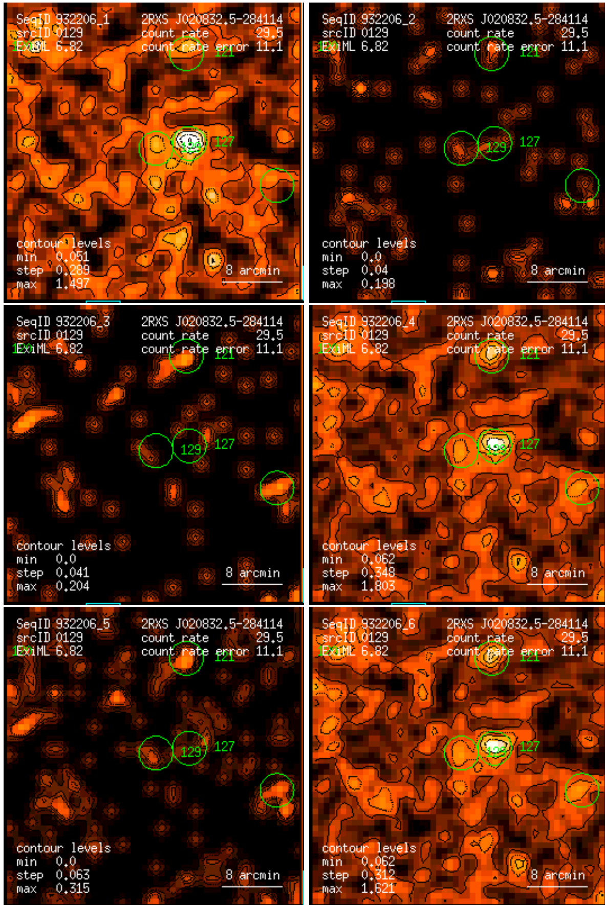
Figure 129: RASS 932206: detection 0129: band rate images, Gaussian filter: (1) PSPC channels 11 – 41, (2) 52 – 90, (3) 91 – 201, (4) 11 – 235, (5) 52 – 201, (6) 11 – 201. Broad band rates in counts/ks. Band rate contour levels in counts/ks/arcmin 2 .
