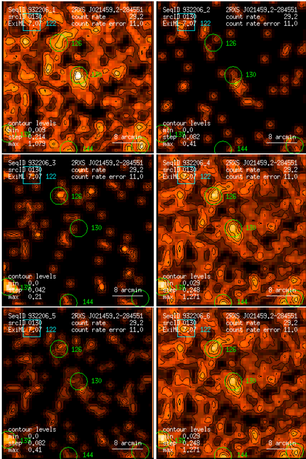
Figure 130: RASS 932206: detection 0130: band rate images, Gaussian filter: (1) PSPC channels 11 – 41, (2) 52 – 90, (3) 91 – 201, (4) 11 – 235, (5) 52 – 201, (6) 11 – 201. Broad band rates in counts/ks. Band rate contour levels in counts/ks/arcmin 2 .
