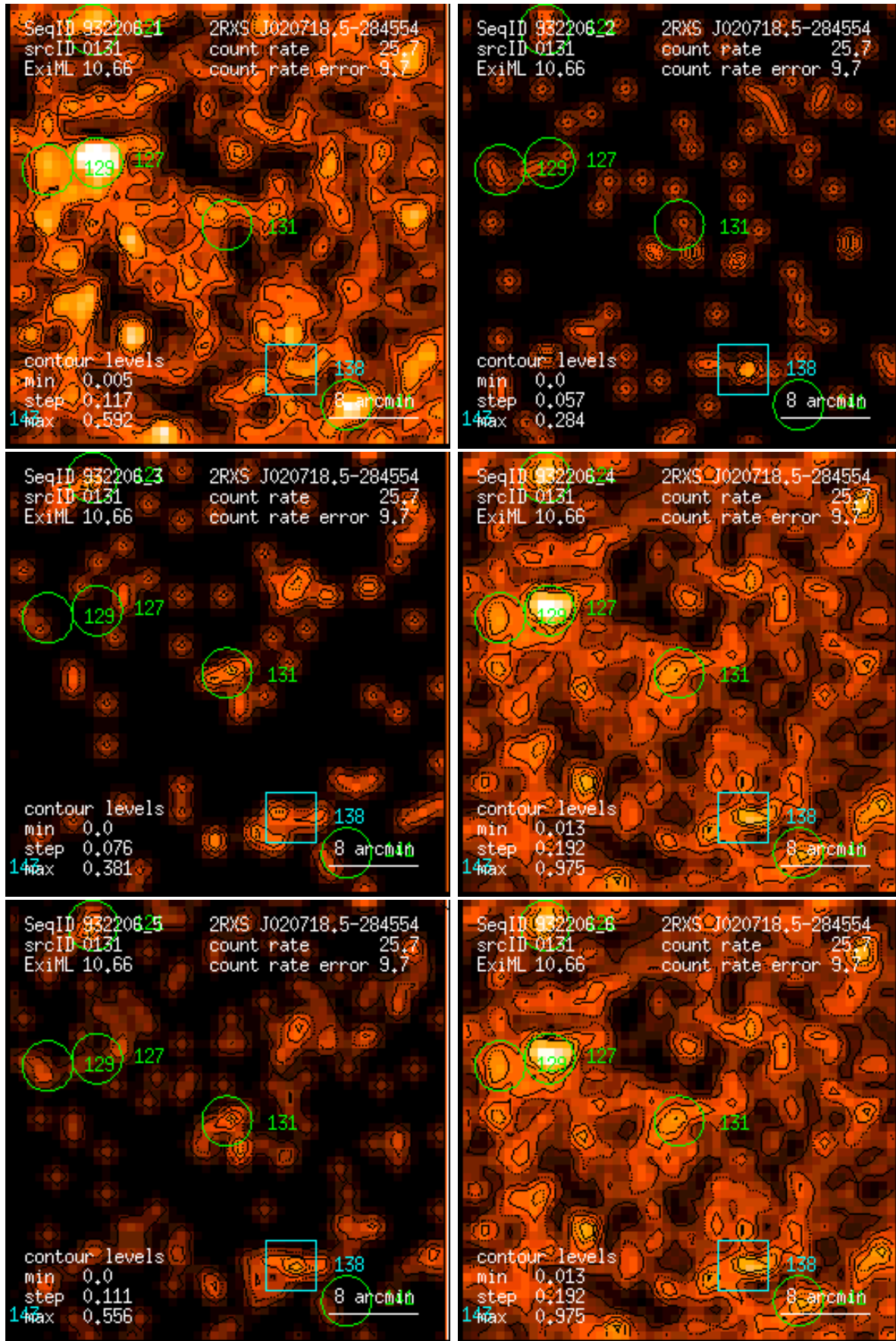
Figure 131: RASS 932206: detection 0131: band rate images, Gaussian filter: (1) PSPC channels 11 – 41, (2) 52 – 90, (3) 91 – 201, (4) 11 – 235, (5) 52 – 201, (6) 11 – 201. Broad band rates in counts/ks. Band rate contour levels in counts/ks/arcmin 2 .
