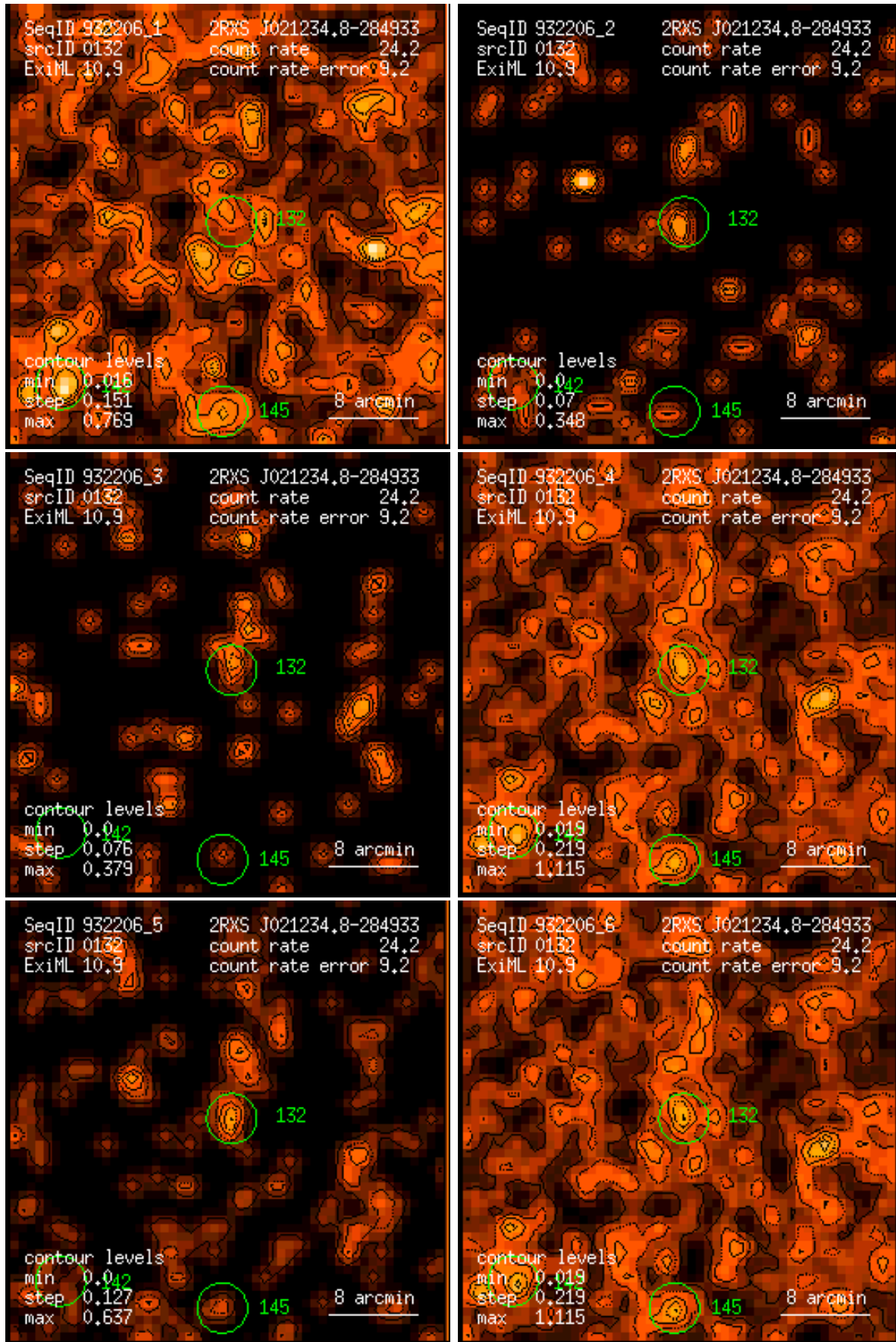
Figure 132: RASS 932206: detection 0132: band rate images, Gaussian filter: (1) PSPC channels 11 – 41, (2) 52 – 90, (3) 91 – 201, (4) 11 – 235, (5) 52 – 201, (6) 11 – 201. Broad band rates in counts/ks. Band rate contour levels in counts/ks/arcmin 2 .
