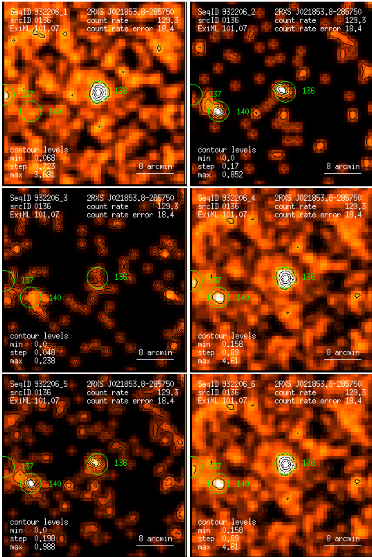
Figure 136: RASS 932206: detection 0136: band rate images, Gaussian filter: (1) PSPC channels 11 – 41, (2) 52 – 90, (3) 91 – 201, (4) 11 – 235, (5) 52 – 201, (6) 11 – 201. Broad band rates in counts/ks. Band rate contour levels in counts/ks/arcmin 2 .
