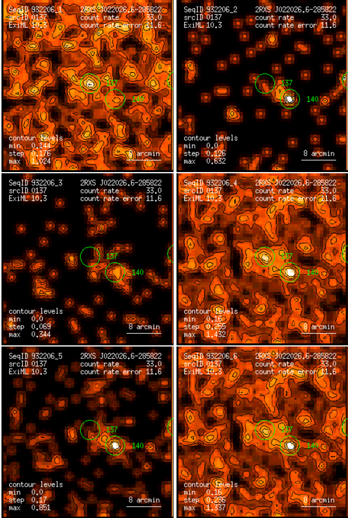
Figure 137: RASS 932206: detection 0137: band rate images, Gaussian filter: (1) PSPC channels 11 – 41, (2) 52 – 90, (3) 91 – 201, (4) 11 – 235, (5) 52 – 201, (6) 11 – 201. Broad band rates in counts/ks. Band rate contour levels in counts/ks/arcmin 2 .
