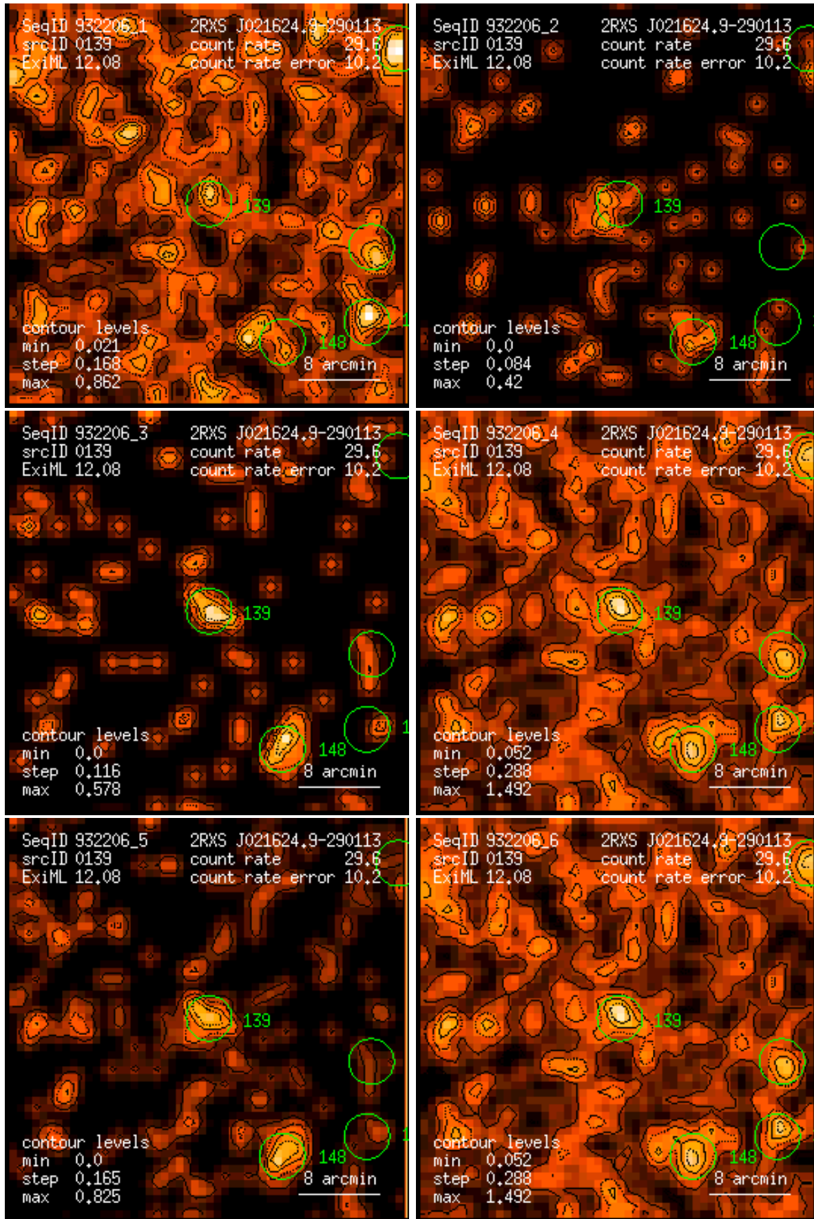
Figure 139: RASS 932206: detection 0139: band rate images, Gaussian filter: (1) PSPC channels 11 – 41, (2) 52 – 90, (3) 91 – 201, (4) 11 – 235, (5) 52 – 201, (6) 11 – 201. Broad band rates in counts/ks. Band rate contour levels in counts/ks/arcmin 2 .
