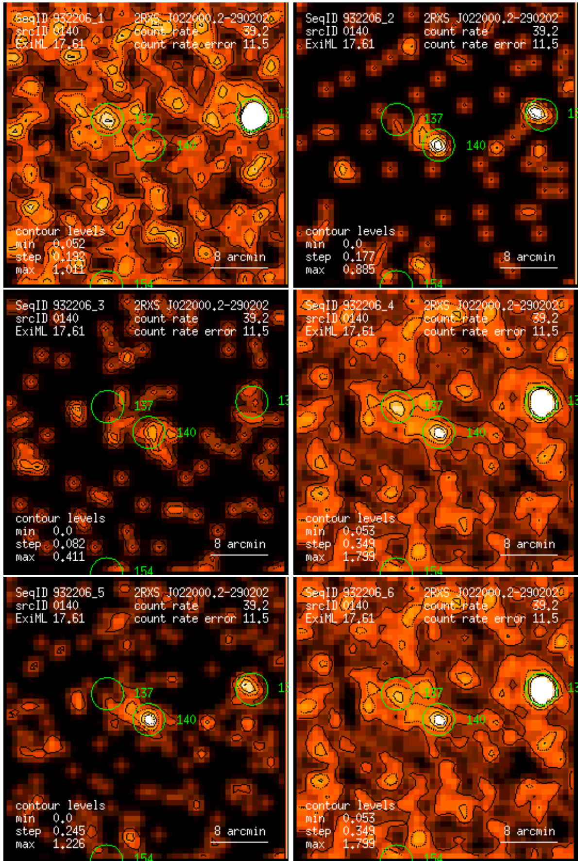
Figure 140: RASS 932206: detection 0140: band rate images, Gaussian filter: (1) PSPC channels 11 – 41, (2) 52 – 90, (3) 91 – 201, (4) 11 – 235, (5) 52 – 201, (6) 11 – 201. Broad band rates in counts/ks. Band rate contour levels in counts/ks/arcmin 2 .
