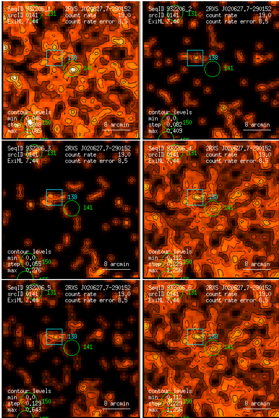
Figure 141: RASS 932206: detection 0141: band rate images, Gaussian filter: (1) PSPC channels 11 – 41, (2) 52 – 90, (3) 91 – 201, (4) 11 – 235, (5) 52 – 201, (6) 11 – 201. Broad band rates in counts/ks. Band rate contour levels in counts/ks/arcmin 2 .
