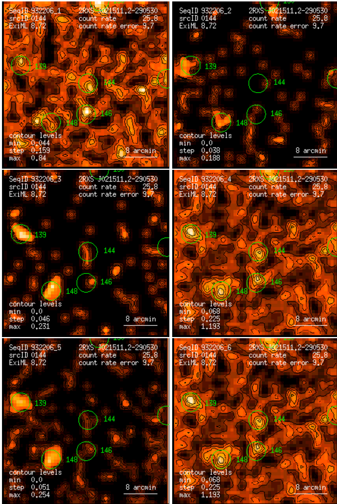
Figure 144: RASS 932206: detection 0144: band rate images, Gaussian filter: (1) PSPC channels 11 – 41, (2) 52 – 90, (3) 91 – 201, (4) 11 – 235, (5) 52 – 201, (6) 11 – 201. Broad band rates in counts/ks. Band rate contour levels in counts/ks/arcmin 2 .
