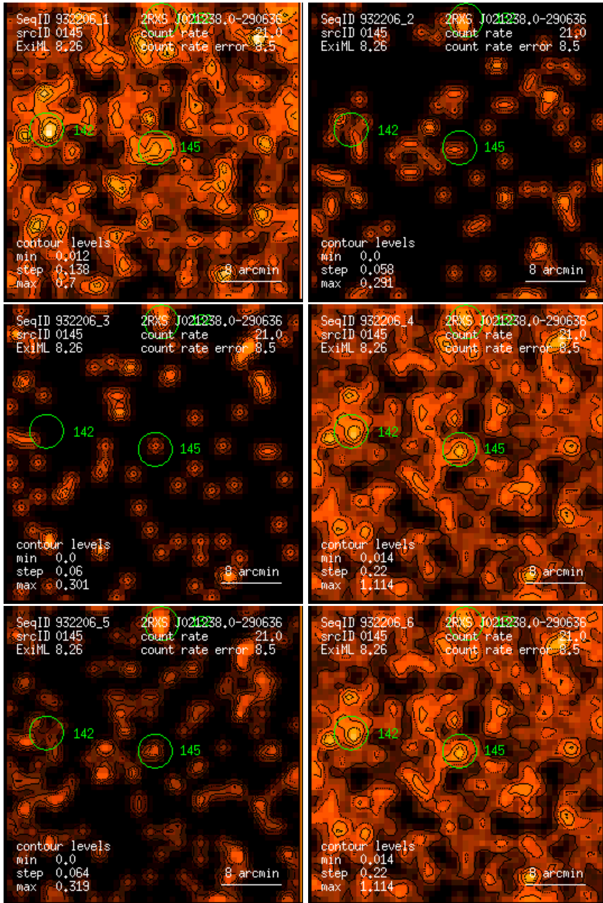
Figure 145: RASS 932206: detection 0145: band rate images, Gaussian filter: (1) PSPC channels 11 – 41, (2) 52 – 90, (3) 91 – 201, (4) 11 – 235, (5) 52 – 201, (6) 11 – 201. Broad band rates in counts/ks. Band rate contour levels in counts/ks/arcmin 2 .
