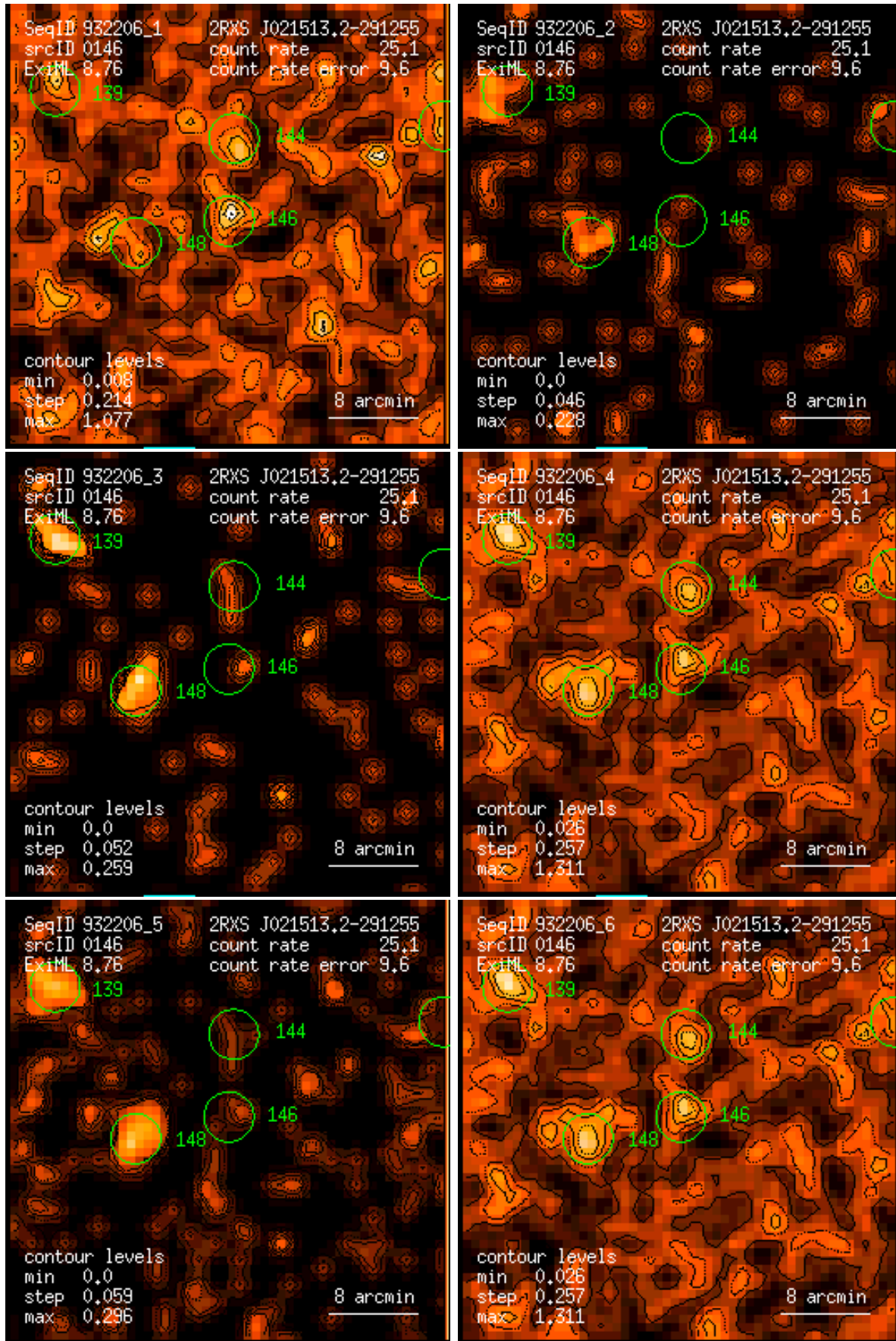
Figure 146: RASS 932206: detection 0146: band rate images, Gaussian filter: (1) PSPC channels 11 – 41, (2) 52 – 90, (3) 91 – 201, (4) 11 – 235, (5) 52 – 201, (6) 11 – 201. Broad band rates in counts/ks. Band rate contour levels in counts/ks/arcmin 2 .
