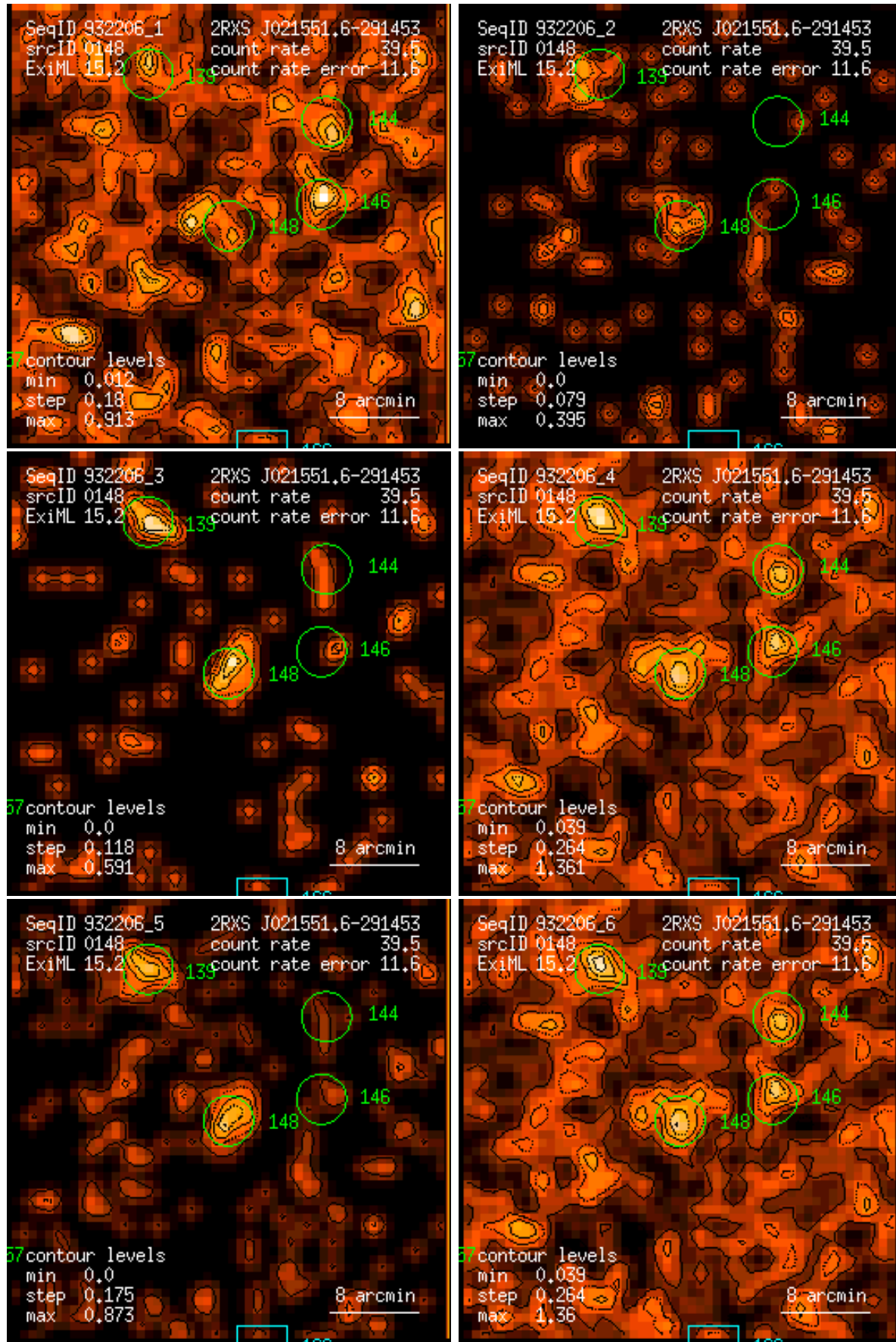
Figure 148: RASS 932206: detection 0148: band rate images, Gaussian filter: (1) PSPC channels 11 – 41, (2) 52 – 90, (3) 91 – 201, (4) 11 – 235, (5) 52 – 201, (6) 11 – 201. Broad band rates in counts/ks. Band rate contour levels in counts/ks/arcmin 2 .
