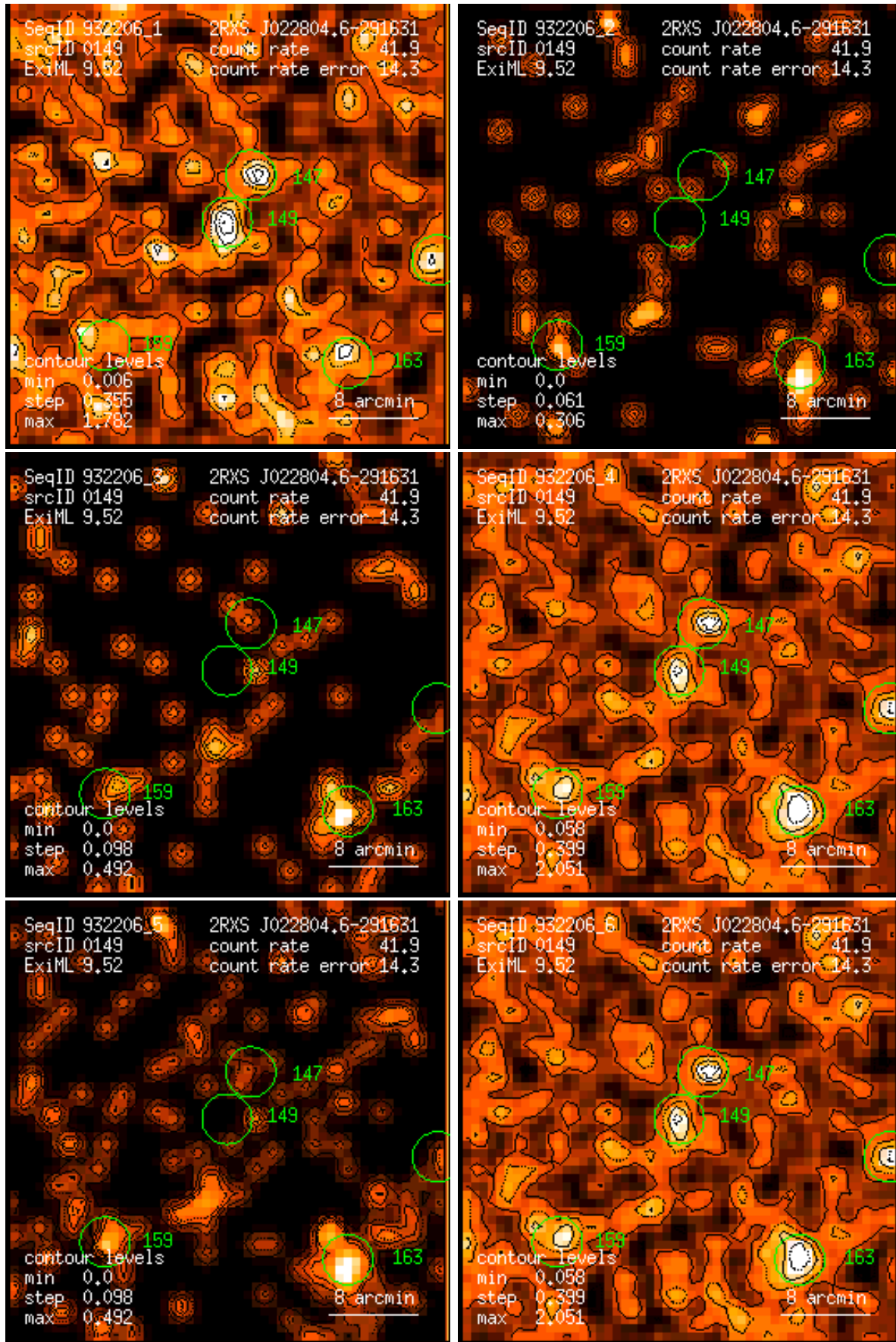
Figure 149: RASS 932206: detection 0149: band rate images, Gaussian filter: (1) PSPC channels 11 – 41, (2) 52 – 90, (3) 91 – 201, (4) 11 – 235, (5) 52 – 201, (6) 11 – 201. Broad band rates in counts/ks. Band rate contour levels in counts/ks/arcmin 2 .
